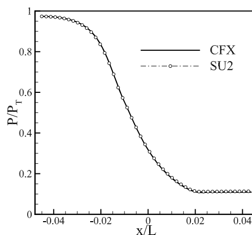
Figure 6: Streamwise distribution of the static pressure at the mid section of the nozzle.
