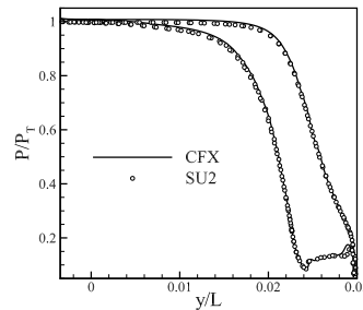
Figure 8: Pressure distribution along the blade surface.
