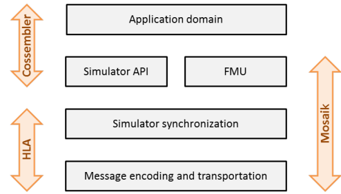
Fig. 1. Cossembler in relationship to other co-simulation architectures.
