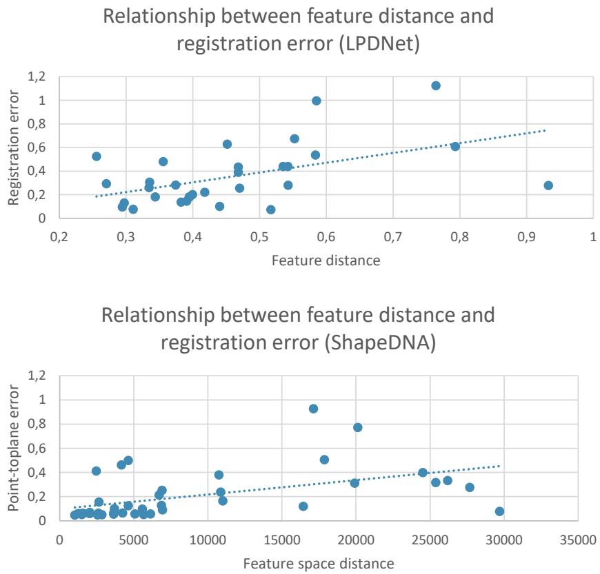
Figure 44: Relationship between descriptor distance in feature space and point-to-plane error after registration.
