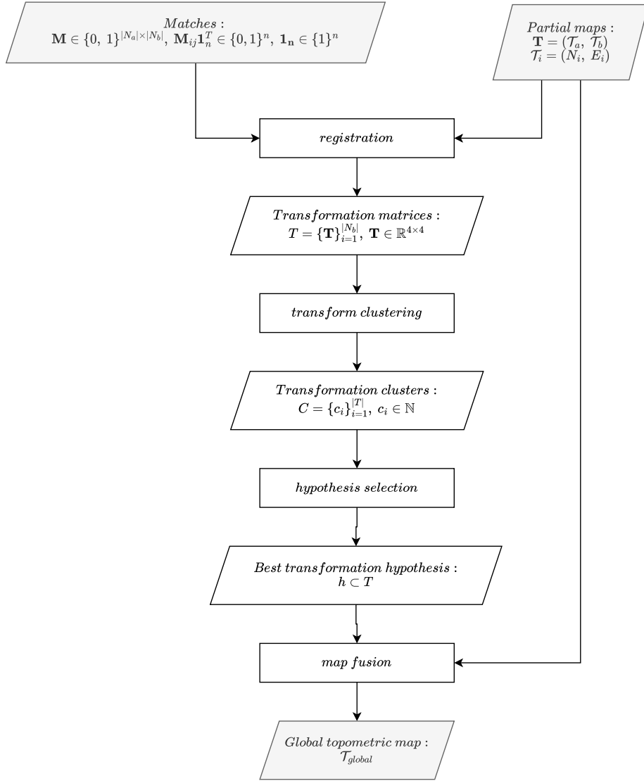
Figure 34: Diagram showing overview of map fusion methodology.
