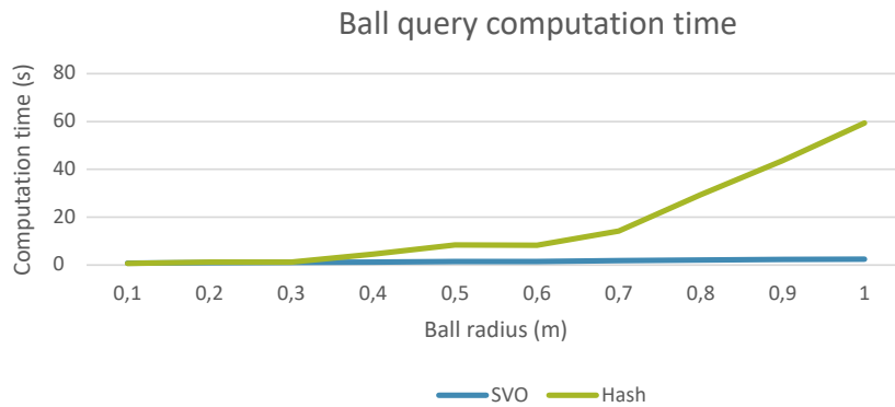
Figure 38: Comparison of SVO radius search performance versus voxel hashing.
