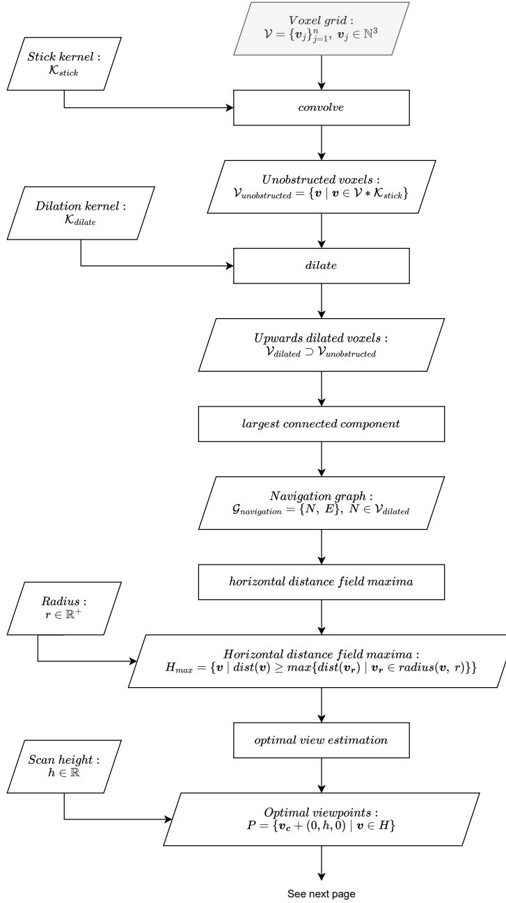
Figure 19: Diagram showing map extraction processes and intermediate data (part 1).
