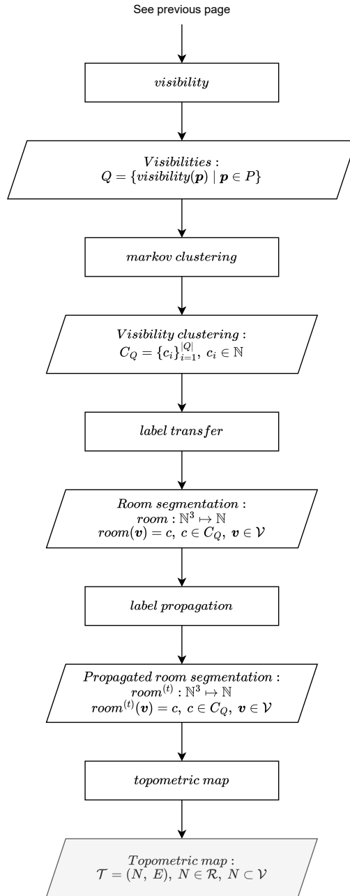
Figure 20: Diagram showing map extraction processes and intermediate data (part 2).
