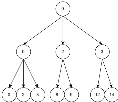
Figure 15: Example of a sparse voxel octree generated from the above Morton codes.
