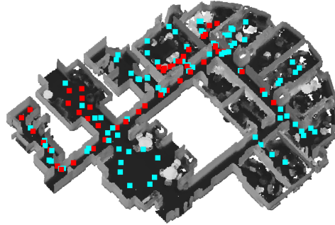
Figure 35: Global map with simulated viewpoints. Each coloured dot represents a viewpoint, the union of all views with the same color forms a partial map.
