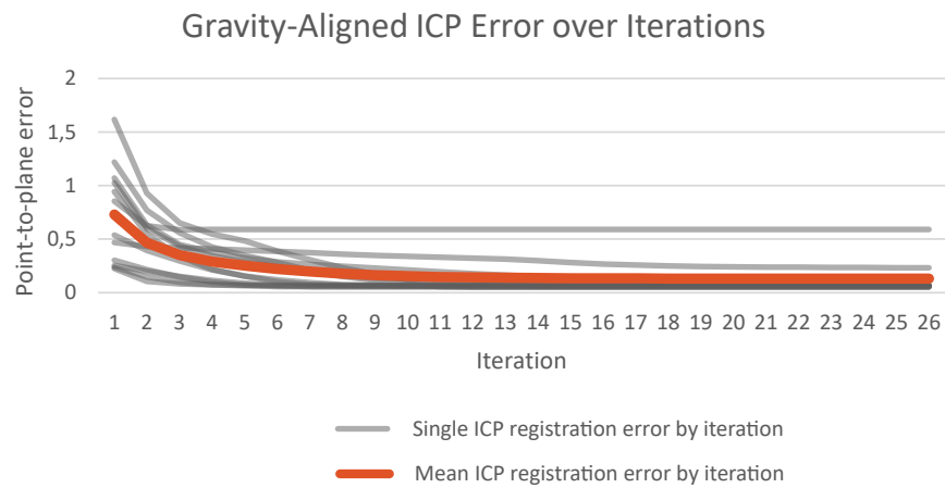
Figure 46: Convergence of ICP algorithm over multiple iterations.
