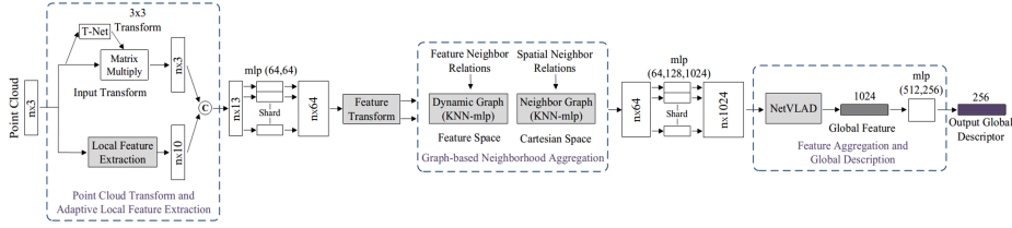
Figure 30: Diagram showing LPDNet network architecture (Z. Liu et al., 2019).
