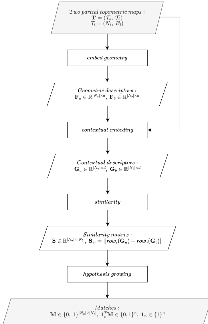
Figure 28: Diagram showing map matching methodology.
