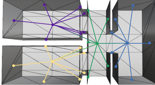
Figure 10: Dual graph of a mesh representation of the environment coloured according to its spectrum ((Bot et al., 2019)).
