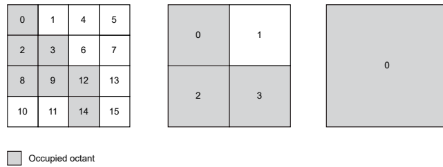
Figure 14: 2D example of morton codes.
