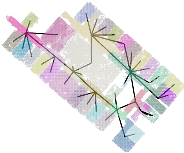
Figure 18: Example of a topometric map.
