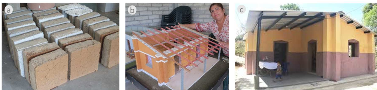
Figure 12. Adobe housing in El Salvador; (a) storage adobe blocks, (b) model earthquake resistant house, (c) built earthquake resistant house. Sources: (a) and (b) Bredenoord; (c) Fundasal.
