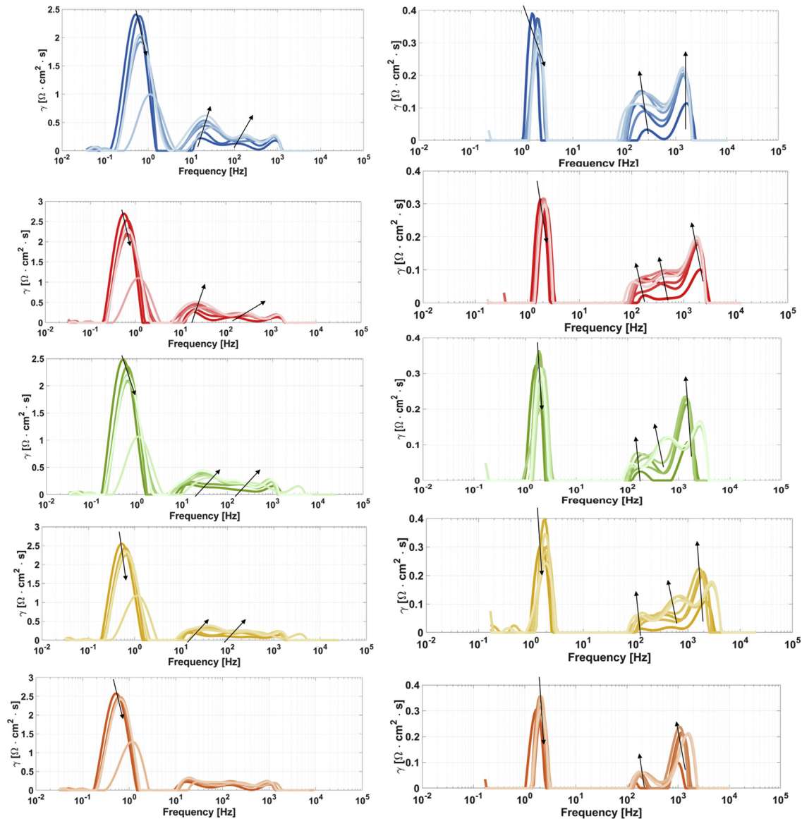
Figure A5 – The distribution of relaxation times for RU1-5 (top to bottom) in SOFC mode (left) and SOEC mode (right) from S1 to S7.
