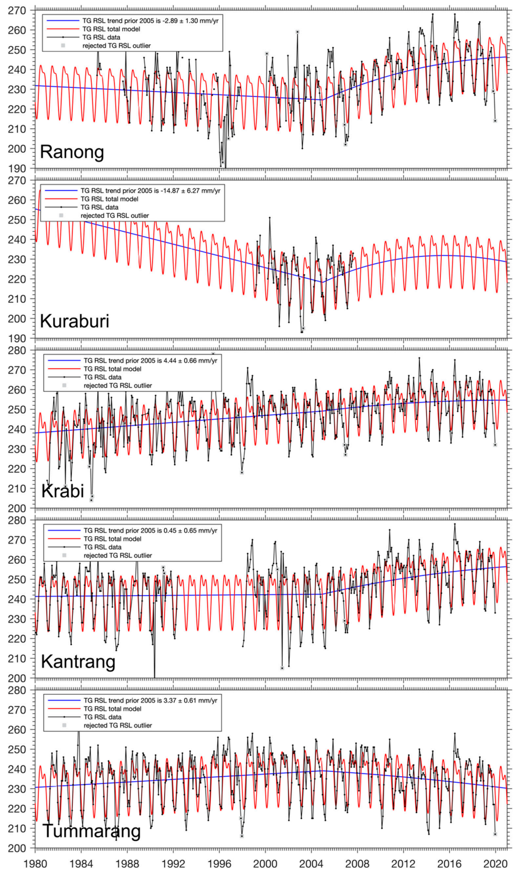
Figure 8. The relative sea-level changes recorded by the TMD TG stations (1980–2020) in the south of Thailand (Y-axis in cm, X-axis in years). Trends are indicated by the blue lines and have been
