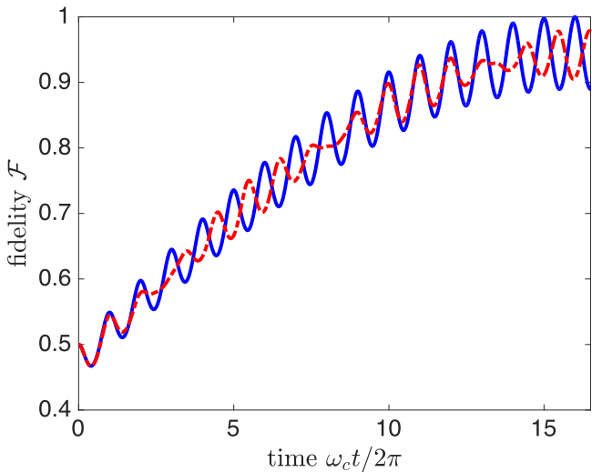
FIG. 13. Fidelity \mathcal{F} = \langle \Psi_{\text{tar}} | \rho_{\text{qubits}} | \Psi_{\text{tar}} \rangle for the two-qubit state \rho_{\text{qubits}} = \text{Tr}_{\text{cav}}[\rho] with the target state |\Psi_{\text{tar}}\rangle = (|\uparrow\downarrow\rangle + i|\downarrow\uparrow\rangle)/\sqrt{2} for both \omega_q/\omega_c = 0 (solid blue line) and \omega_q/\omega_c = 0.1 (dashed red line); here, g/\omega_c = \frac{1}{16} < 0.1 . Other numerical parameters: k_B T/\omega_c = 2 ( \bar{n}_{\text{th}} \approx 1.54 ), Q = 10^5 , and \Gamma/\omega_c = 0 .
