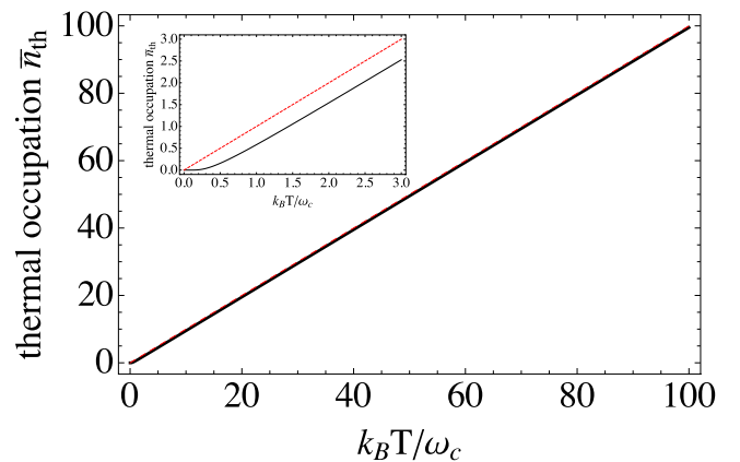
FIG. 5. Thermal occupation \bar{n}_{\text{th}} = (\exp[\hbar\omega_c/k_B T] - 1)^{-1} (black solid line) and high-temperature approximate result \bar{n}_{\text{th}} \approx k_B T/\hbar\omega_c (red dashed line). For T = 4 K and \omega_c/2\pi = 1 GHz ( \omega_c/2\pi = 10 GHz), we have k_B T/\hbar\omega_c \approx 80 ( k_B T/\hbar\omega_c \approx 8 ). For T = 1 K and \omega_c/2\pi = 1 GHz ( \omega_c/2\pi = 10 GHz), we have \bar{n}_{\text{th}} \approx 20 ( \bar{n}_{\text{th}} \approx 2 ).
