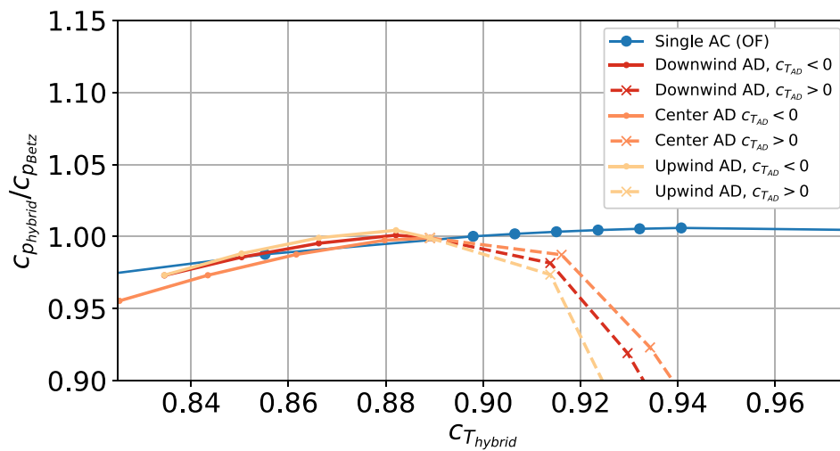
FIGURE 12 Power coefficient of an idealized hybrid VAWT c_{p_{hybrid}}/c_{p_{Betz}} with varied c_{TAD} , c_{TAC} = 0.89 . VAWT, vertical axis wind turbine.
