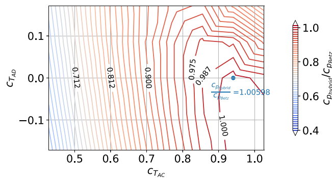
FIGURE 13 Power coefficient of an idealized hybrid VAWT c_{p_{hybrid}}/c_{p_{Betz}} with downwind AD for different combinations of c_{TAD} and c_{TAC} . AD, actuator disk; VAWT, vertical axis wind turbine.
