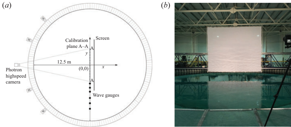
Figure 2. Experimental set-up with (a) diagram of the wave tank, showing wave gauge array A, Qualisys infra-red (IR) cameras, high-speed camera, calibration plane and screen; and (b) photograph of the wave tank and the screen.
