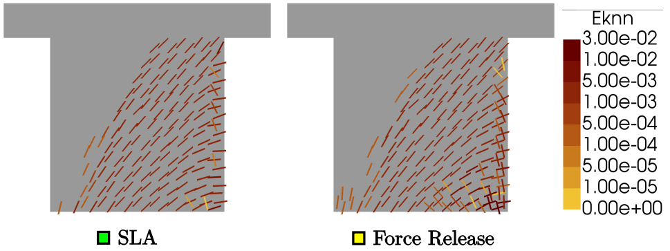
Figure 4.12: Crack pattern plots (E knn denotes the normal crack strain) of SLA & Force-Release simulations of the RC shear wall experiment at the onset of collapse. (refer Figure 4.8) (Splitting cracks at the toe captured better in Force-Release compared to SLA)
