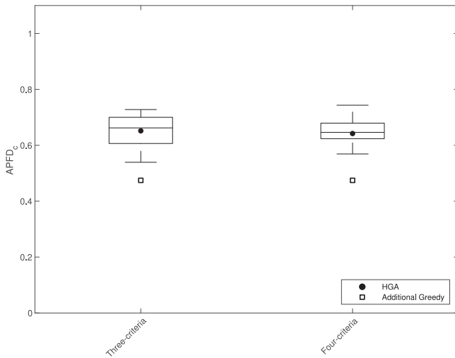
Fig. 9. APFD c scores achieved by Additional Greedy (□), GA (*), NSGA-II (boxplots), and HGA (●) for MySQL.
