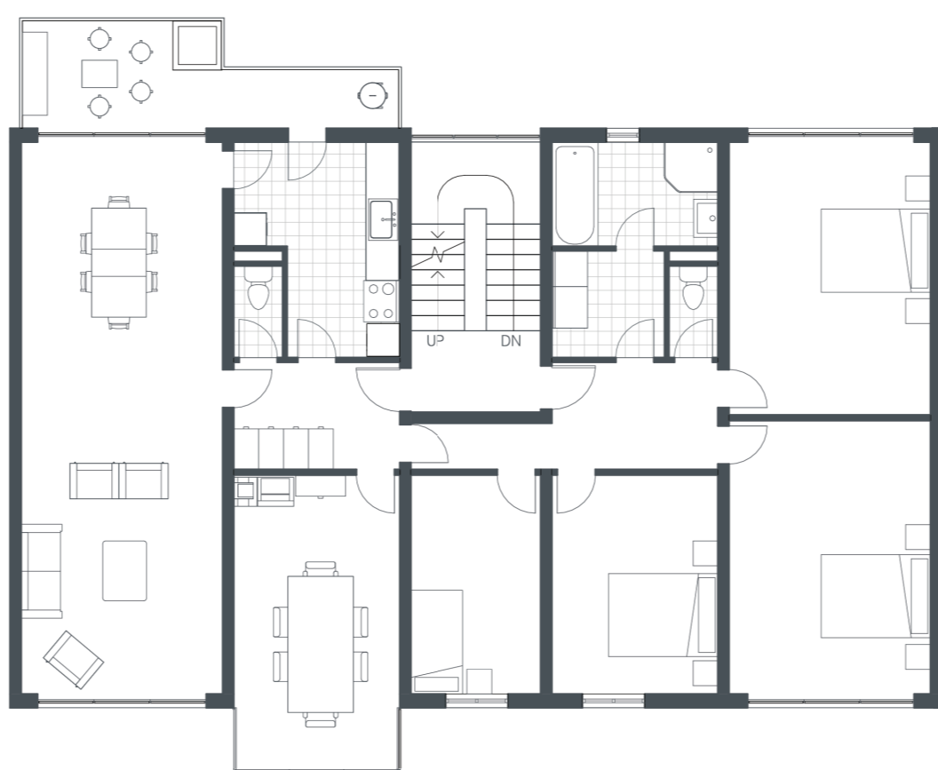
Renovation Office Garden Typology Second to Fourth Floor
