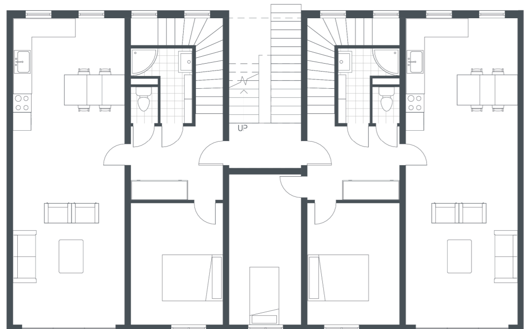
Renovation Mezzanine First Floor
