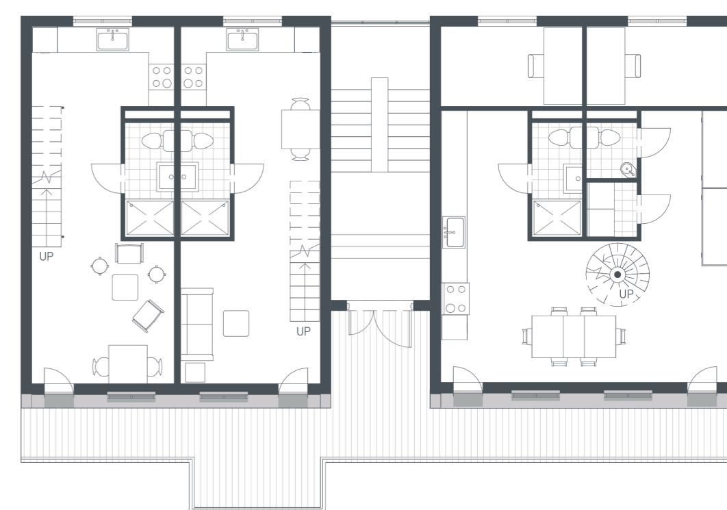
Renovation Optopping Fifth Floor
