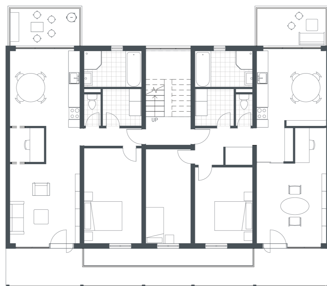
Renovation Gallery Typology Second to Fourth Floor
