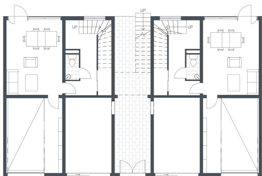
Renovation Mezzanine Ground Floor
