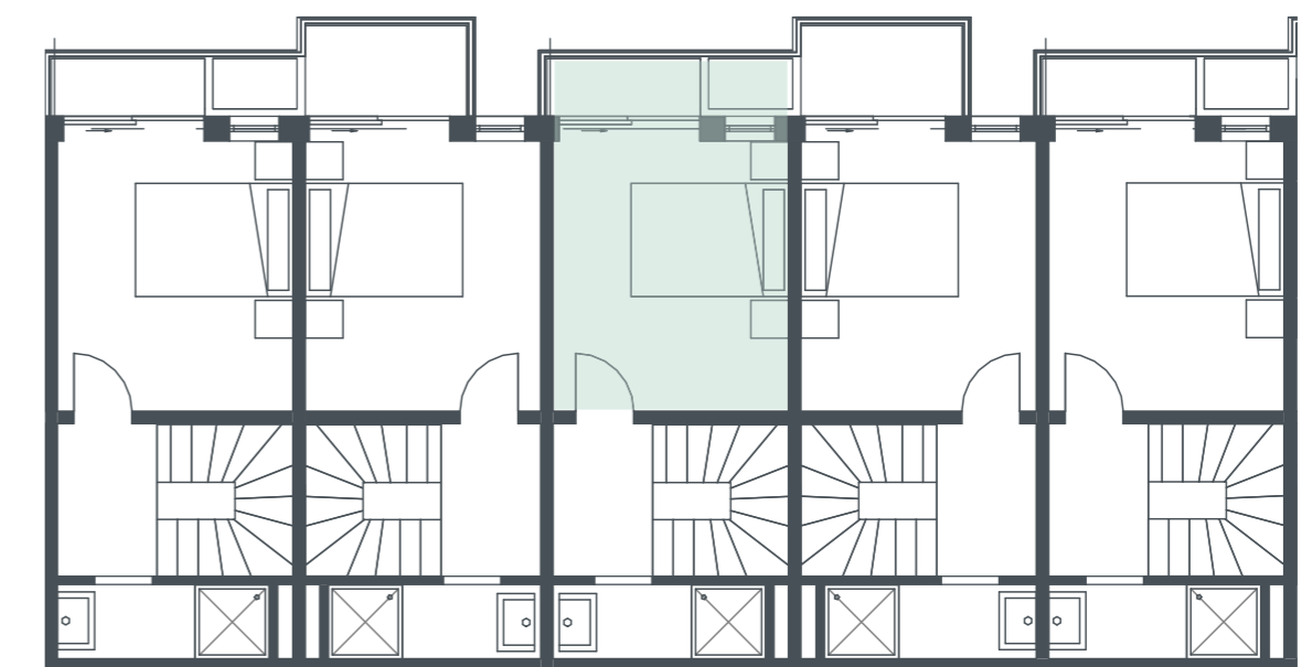
New Co-Housing Third Floor
