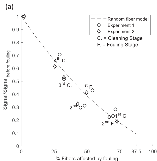
Fig. 7. Shows the correlation between the signal obtained for the |S(k)|^2 coherence peak from the centre-line of k-space plotted against the % of fibers with greater than 5% reduction in volumetric flow which is fibers assessed from velocity images (see (Yan et al., 2023) for reference). For comparison the same correlation for the Monte Carlo model ( n = 50 ) is shown for random fiber fouling (black dash line). It can be seen that there is a strong correlation between % fibers affected by fouling and the magnitude of the coherence peak. Experiment 1 & 2 are detailed in Section 3.1; They consist of two experimental runs, where in each run the module experiences two doses of alginate fouling (1st and 2nd fouling stage) followed by four cleaning stages using pH = 11 NaOH solution (1 st C: flash cleaning; 2 nd C: 20 min soak cleaning; 3 rd C: 1 h soak cleaning and 4 th C: 10 h soak cleaning).
