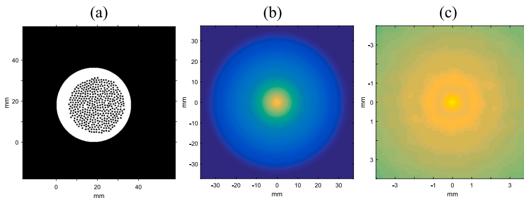
Fig. 3. Shows (a) model MRI image (binary values), (b) NMR Patterson function, (c) zoom-in plot of (b). The nearest neighbour ring seen in the Patterson function is at \sim 1.2 mm (consistent with the outer diameter of the closely packed fibers).
