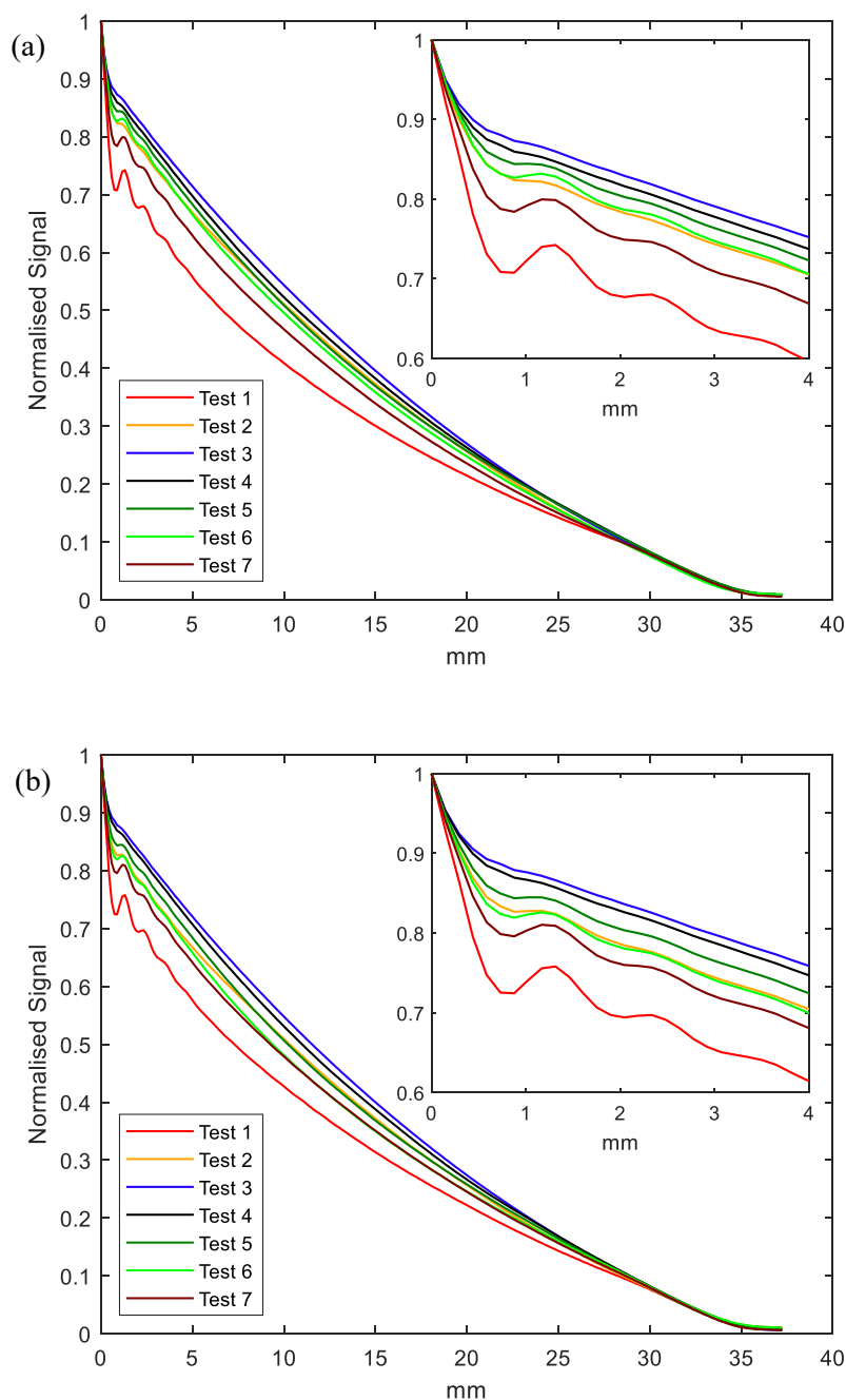
Fig. 5. Shows plots of the radial integral of the Patterson functions obtained during the fouling/cleaning cycle of a membrane module – (a) Experiment 1 and (b) Experiment 2. See S2 and S3 in supplementary material for MRI and Patterson functions for all seven tests. Insert plots show the initial 4 mm length scale to better show the coherence peaks in the data. A minimum is seen at \sim 0.9 mm. Corresponding to the nearest neighbour's coherence structure. As fouling progresses (Test 1 to Test 3) there is a loss in diffraction peak, while during progressive cleaning (Test 4 to Test 7) there is a re-emergence of the coherence peak, however due to residual fouling it does not return to its original shape.
