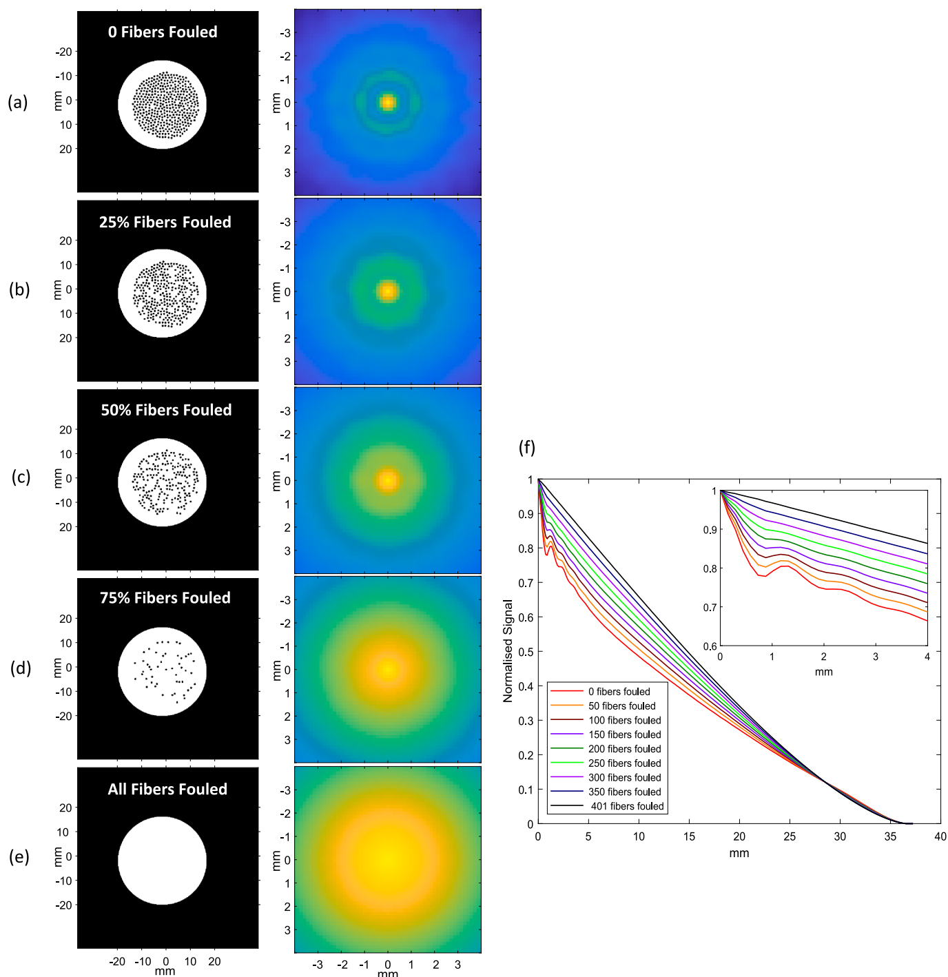
Fig. 4. Simulated MRI module images (left) and Patterson functions (right) for (a) to (e): 0, 100, 200, 300 and 401 fouled fibers. The nearest neighbour diffraction pattern seen in (a) disappears as more fibers are fouled. (f) shows the radial integral of the full Patterson function (0–40 mm), averaged over 50 model runs, with the insert image showing the central region of the Patterson function (0–4 mm). See S1 in supplementary material for model MRI and Patterson functions for all nine fouling cases modelled (from 0 to 401 fibers fouled in increments of 50 fibers).
