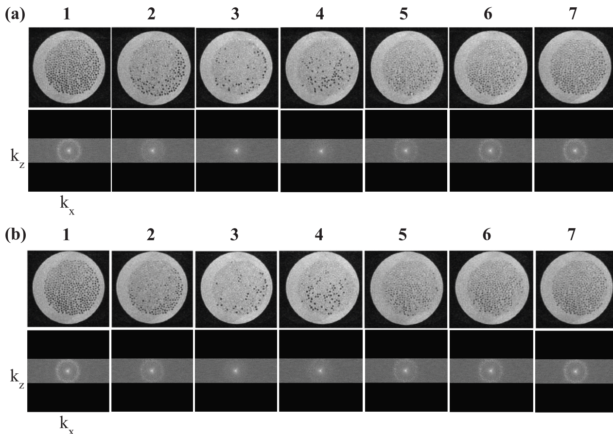
Fig. 2. MRI images (top row) and k -space images (bottom row) with flow encoding gradient obtained during the fouling/cleaning cycle of a membrane module – (a) Experiment 1 and (b) Experiment 2. k -space plot is plotted using absolute values on \log_{10} scale, while the MRIs show membrane region (see supplementary material for full MRIs) – this is to better visualise the k -space coherence ring structure, and ease visual comparison with the membrane region in MRIs as the coherence ring structure disappears and re-appears while system is fouled (1–3) and cleaned (4–7). The x and z represent read encode direction and phase encode direction respectively. The images are acquired 40 mm from the fiber's entrance manifold.
