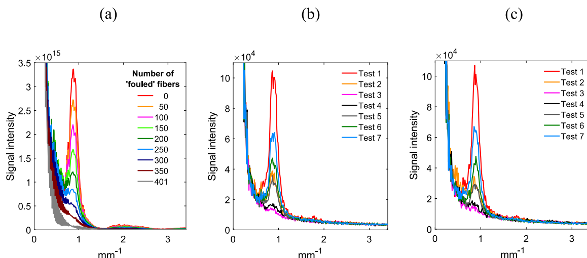
Fig. 6. (a) Model result for the radial integration of |S(k)|^2 function as the number of 'fouled' fibers increases – with the location of fibers determined randomly. (b) and (c) Experimental |S(k)|^2 results for the 1st and 2nd experimental fouling/cleaning cycles. The coherence feature largely disappears at the 2nd fouling (Test 3) and 1st cleaning (Test 4) stage – indicative of ineffective cleaning – whilst subsequent cleaning results in the gradual recovery of the feature (Test 5 to Test 7). It is notable that the feature is quite a bit lower in Test 7 than Test 1, indicating that there is residual fouling in the module even after 10 h or NaOH soaking.
