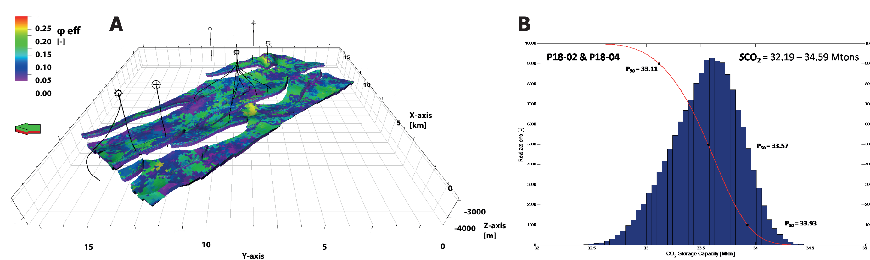
Fig 4 A) Static reservoir model of the effective porosity distribution in the P18 field. B) Results of Monte-Carlo simulations of the modelled reservoir capacity.
