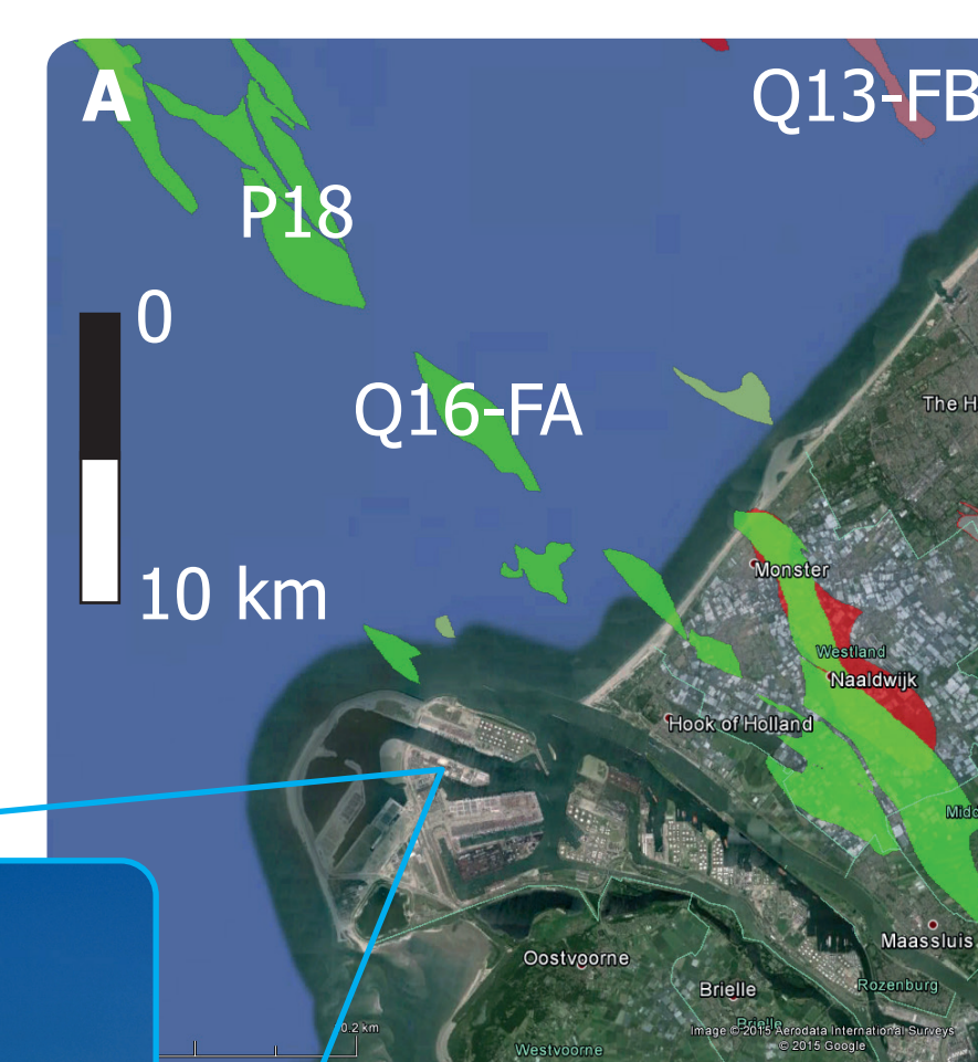
Fig. 2 A) Overlay of oil and gas fields on Google Earth image (north is up). B) E.ON MPP3 power plant.
