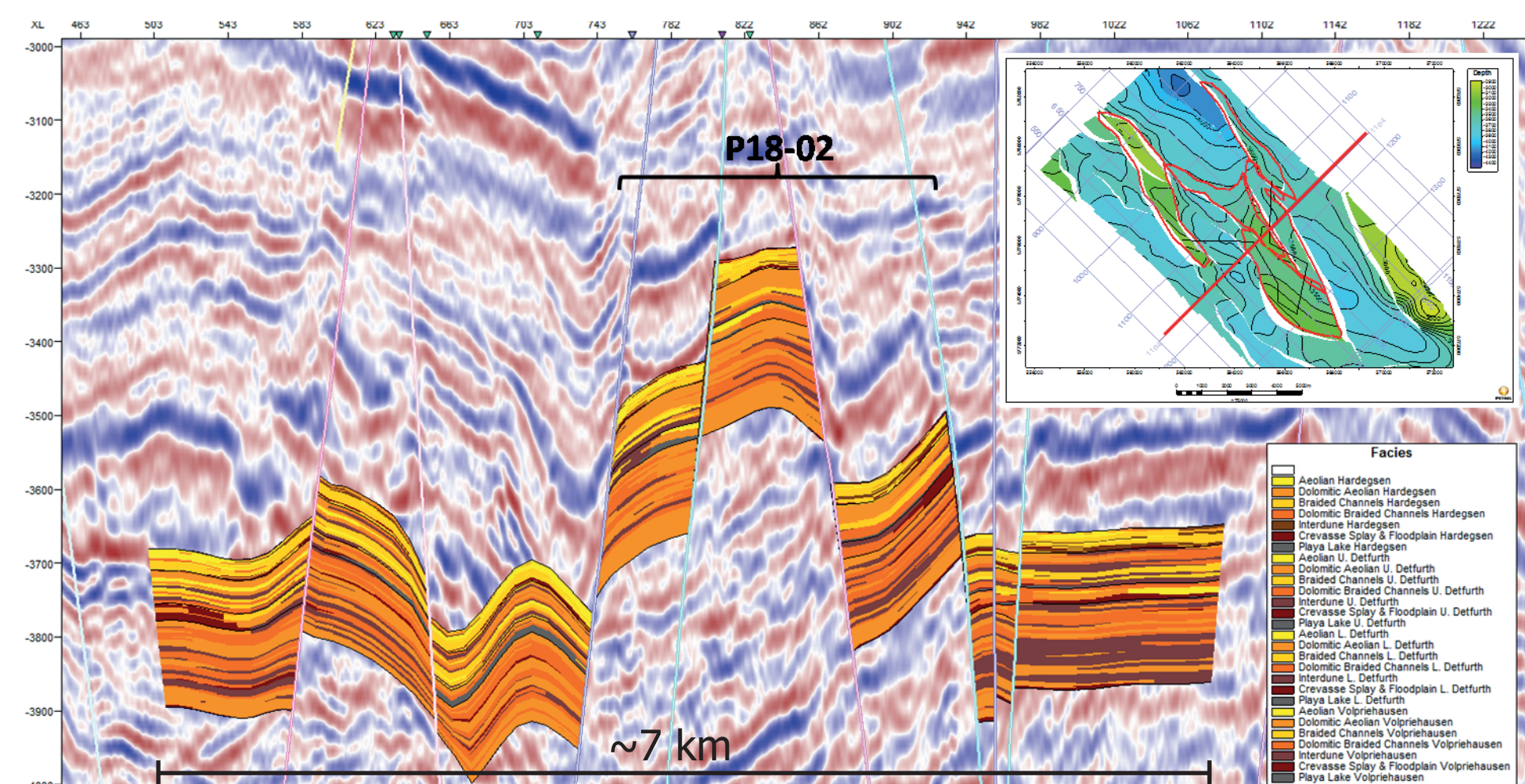
Fig. 3 Seismic inline through the P18 field (NE-SW; inset top right) showing interpreted faults and the facies model of the reservoir interval. Note that juxtaposition may isolate fault-bounded compartments.
