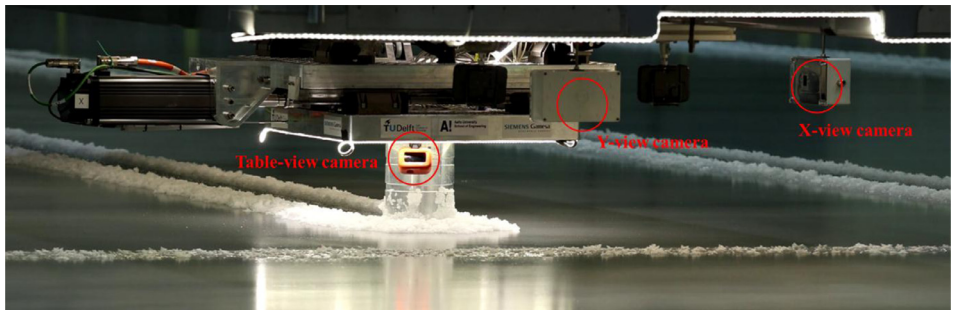
Fig. 12. Cameras capturing the ice-structure interaction from different viewpoints.
