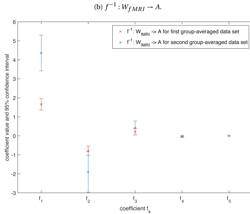
Figure 5.5: (a) Estimated coefficients for the mapping f^{-1} : W_{MEG} \rightarrow A for K = 5 together with their 95% confidence interval for the first group-averaged data set and a second group-averaged data set. (b) Estimated coefficients for the mapping f^{-1} : W_{fMRI} \rightarrow A for K = 5 together with their 95% confidence interval for the first group-averaged data set and a second group-averaged data set.
