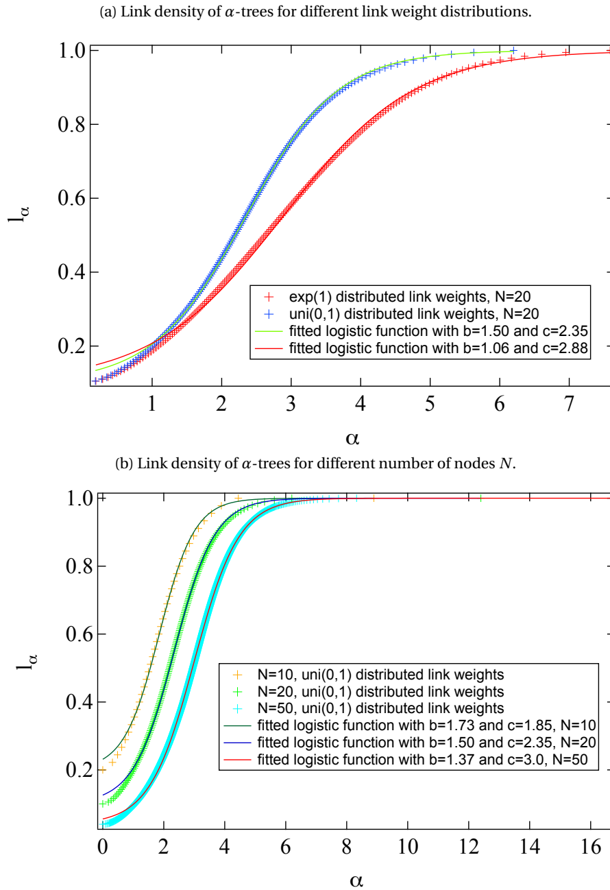
Figure 3.3: (a) The link density l_\alpha of the \alpha -tree versus \alpha for 10^4 realizations of networks with N = 20 nodes, both for exponentially distributed link weights with mean 1 and uniformly distributed link weights in the interval (0, 1) . (b) The link density l_\alpha versus \alpha for 10^4 realizations of networks with N = 10, 20 and 50 nodes for uniformly distributed link weights between 0 and 1 . All curves were fitted with the function in Eq. (3.2) with a least-squared fitting procedure. For bigger N , the parameter b of the logistic function in Eq. (3.2), which represents the steepness of the function, decreases while the parameter c , the midpoint of the growth, increases. Except for the values of \alpha < 1 , the fitted function describes the development quite accurately. The discrepancies for small values of \alpha probably originate from numerical imprecision.
