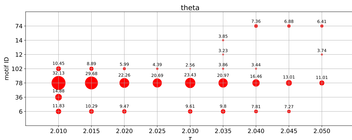
Figure 4.10: Overexpressed 3-motifs for theta frequency band data in the interval [\tau_{min}, \tau_{max}] . The area of the circles scales with the z -score. The numerical value of the z -score is plotted on top of each circle for better comparison.
