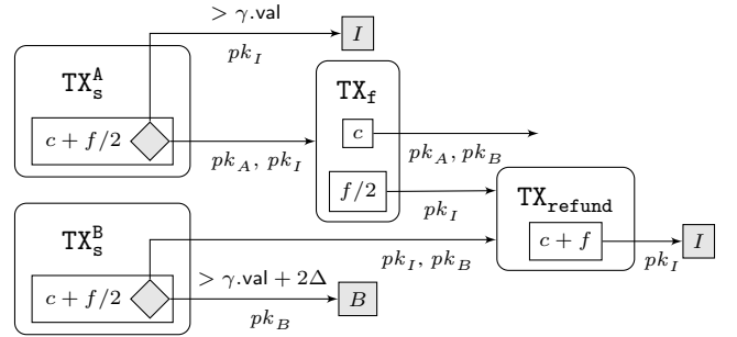
Fig. 12: Funding of a virtual channel \gamma with validity \gamma.\text{val} .
