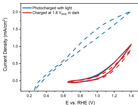
Supplementary Figure S3.7: Cyclic voltammetry of the BiVO 4 sample treated with an anodic potential in the dark for a prolonged time. Cyclic voltammetry of a photocharged BiVO 4 sample is shown for reference. Solid lines represent voltammeteries before the treatment and dotted line represent voltammeteries after the treatment
