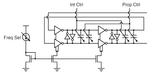
Fig. 3. Ring oscillator.
