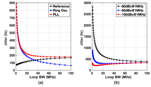
Fig. 6. (a) PLL, VCO and reference jitter versus loop bandwidth, and (b) PLL jitter versus loop bandwidth for VCO phase noises of -80dBc/Hz , -90dBc/Hz , and -100dBc/Hz at 1MHz offset frequency.
