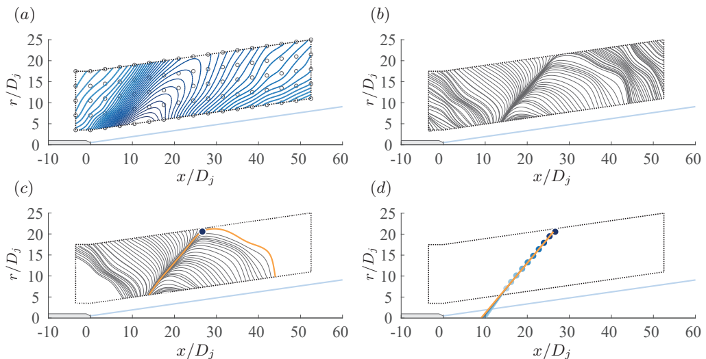
FIGURE 8. (a) Spatial map of \text{SPSL}_{10}(x, r; \text{St}_{10}) , with \text{St}_{10} \approx 0.20 , captured using microphone-array \mathcal{B} . The highest contour level corresponds to 112 dB, residing closest to the shear layer, while each subsequent contour is -1 dB. (b) Perpendicular gradient-field lines of the SPSL contour in sub-figure (a). (c) Identification of the gradient-field line that tracks the ridge in the SPSL contour. (d) Linear fits to the gradient-field line of sub-figure (c).
