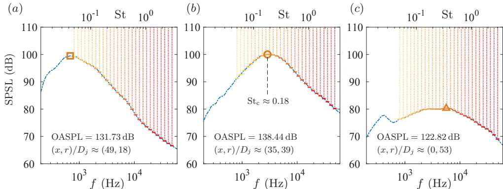
FIGURE 7. (a-c) Sound pressure spectra using (2.5), at three unique grid points. The locations of these points are listed in each sub-figure, and are identified by square, round and triangle shaped markers in Figure 5, respectively.)
