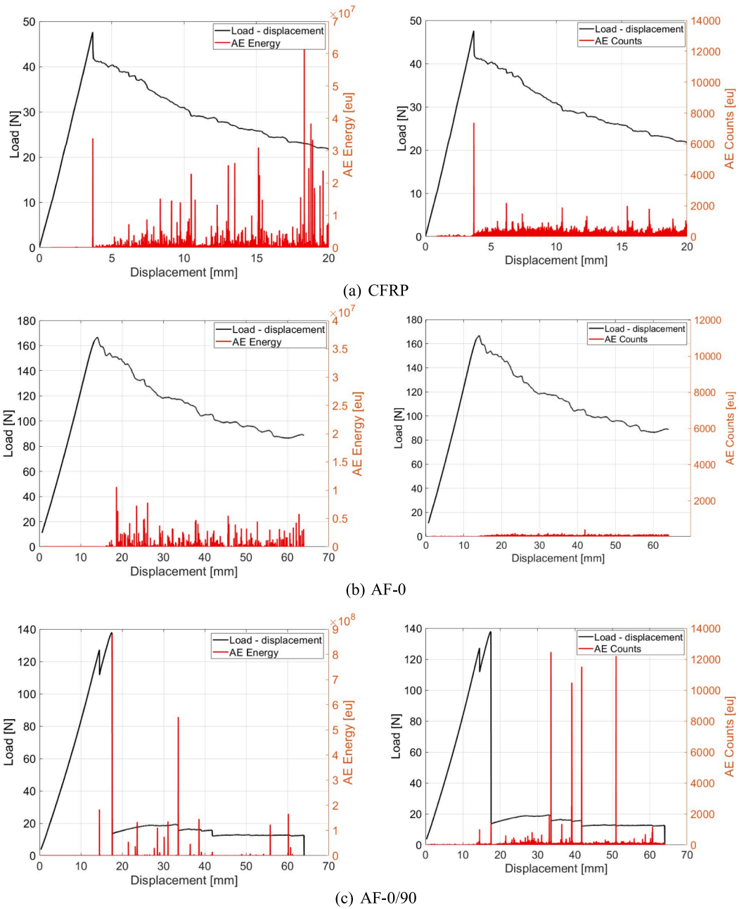
Fig. A.2. Acoustic emission energy raw data and counts related to the load-displacement curve for (a) 0^\circ unidirectional DCB, (b) [0]_8 _AF 163-2 k, (c) [0/90/2/0] S_AF 163-2 k, (d) [90/02/90] S_AF 163-2 k, (e) [90/45/-45/0] S_AF 163-2 k and (f) [90/60/90/-60/0] S_AF 163-2 k specimens.
