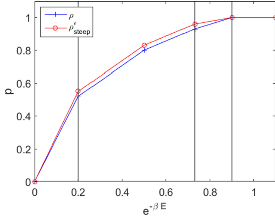
FIG. 6. The thermomajorization diagram divided up into four different regions. In this example, k = 4 . The ordered eigenvalues of \rho and \rho_{\text{st}}^\varepsilon are given by \{0.52, 0.28, 0.13, 0.07, 0\} and \{0.55, 0.28, 0.13, 0.04, 0\} respectively, and their \beta factors by \{0.2, 0.3, 0.23, 0.17, 0.2\} , with \varepsilon = 0.03 .
