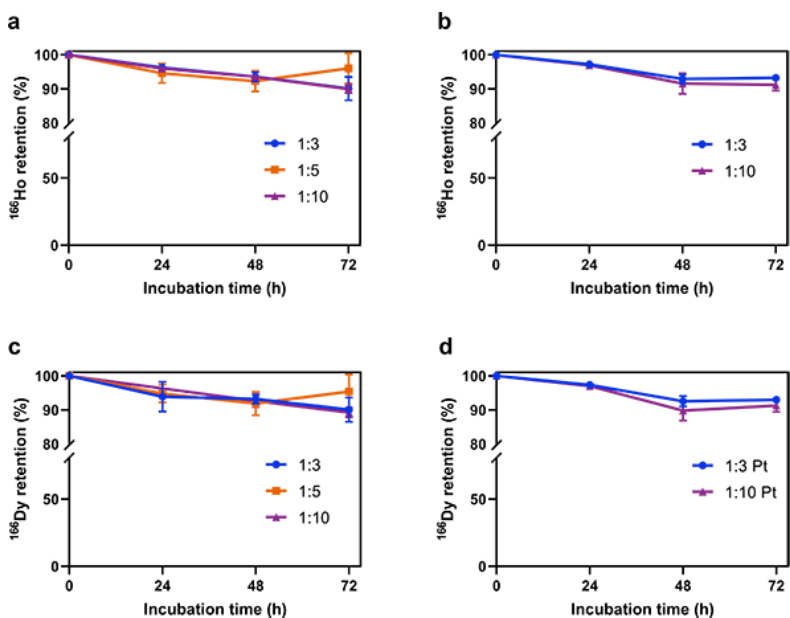
Figure 2.7. ^{166}\text{Ho} and ^{166}\text{Dy} retention of ^{166}\text{DyAu@AuNPs} (a, c) and ^{166}\text{DyPtAuNPs} (b, d) with different Dy:PtAu feeding ratios in 2.5 mM DTPA at 37 °C as function of time. The error bars represent the standard deviation of three independent experiments.
