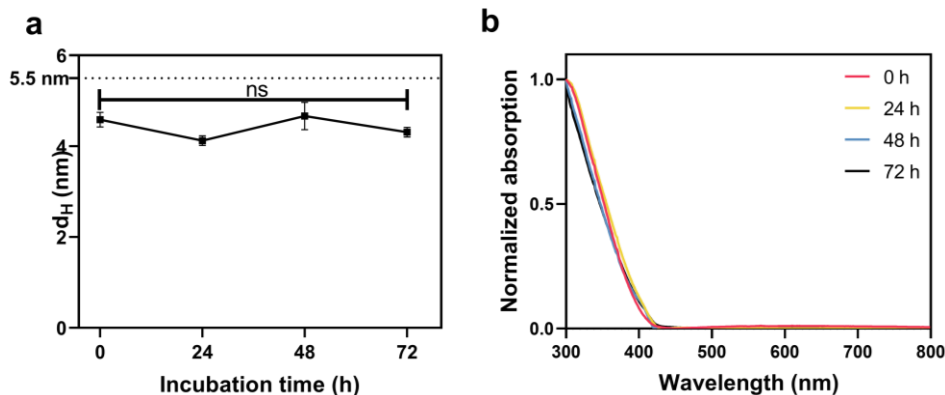
Figure 3.2. Colloidal stability of PEG-AuNPs: a) the number weighted hydrodynamic diameter of PEG-AuNPs in PBS at 37 °C as a function of time, n=3; b) Normalized UV-vis spectrum of PEG-AuNPs in 10% FBS at 37 °C and at different time points.
