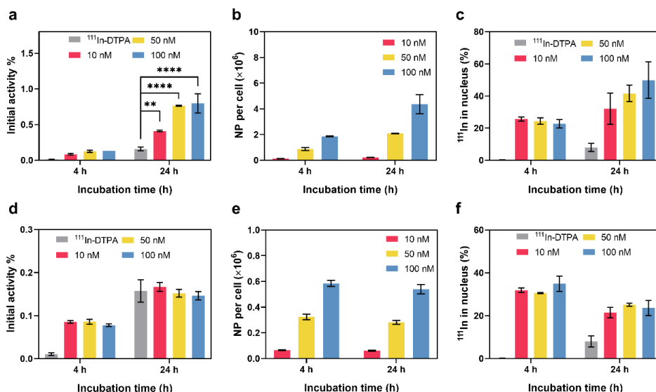
Figure 4.5. In vitro uptake of ^{111}\text{In} -DTPA-AuNPs (a-c) and ^{111}\text{In} -DTPA- \text{Ag}_2\text{Te} NPs (d-f) in 2D U87 cells with various nanoparticle concentrations and an incubation time of 4 or 24 h. a) and d) uptake of ^{111}\text{In} -DTPA-AuNPs and ^{111}\text{In} -DTPA- \text{Ag}_2\text{Te} NPs in U87 cell monolayers. The uptake of ^{111}\text{In} -DTPA using the same ^{111}\text{In} activity was also measured for comparison. The results are presented as percentage of the initially added activity, n=3 ; b) and e) number of internalized ^{111}\text{In} -DTPA-AuNPs and ^{111}\text{In} -DTPA- \text{Ag}_2\text{Te} NPs per cell, n=3 ; c) and f) percentage of ^{111}\text{In} -DTPA-AuNPs and ^{111}\text{In} -DTPA- \text{Ag}_2\text{Te} NPs accumulated in cell nucleus determined by sub-cellular fractionation, n=3 .
