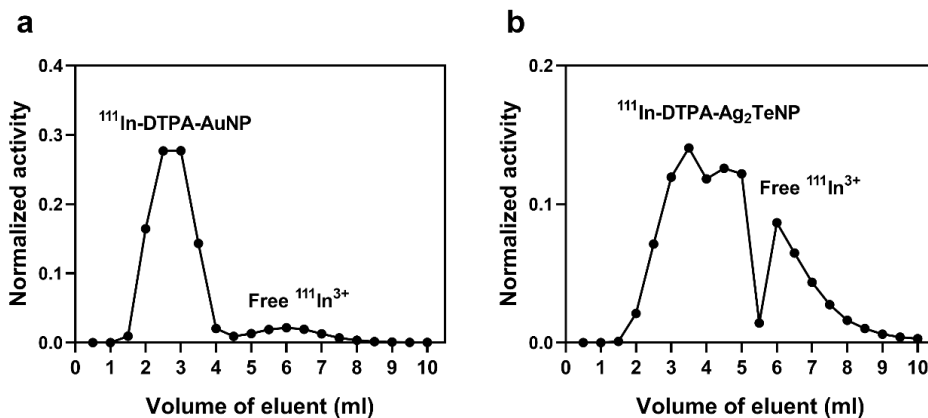
Figure S4.4. Typical elution profiles of a) ^{111}\text{In} -DTPA-AuNPs and b) ^{111}\text{In} -DTPA- \text{Ag}_2\text{Te} NPs in PD-10 columns using PBS as eluent. Fractions were collected every 500 \mu\text{l} . The counts of each fraction were measured with an automated gamma counter for 5 min to collect high enough counts.
