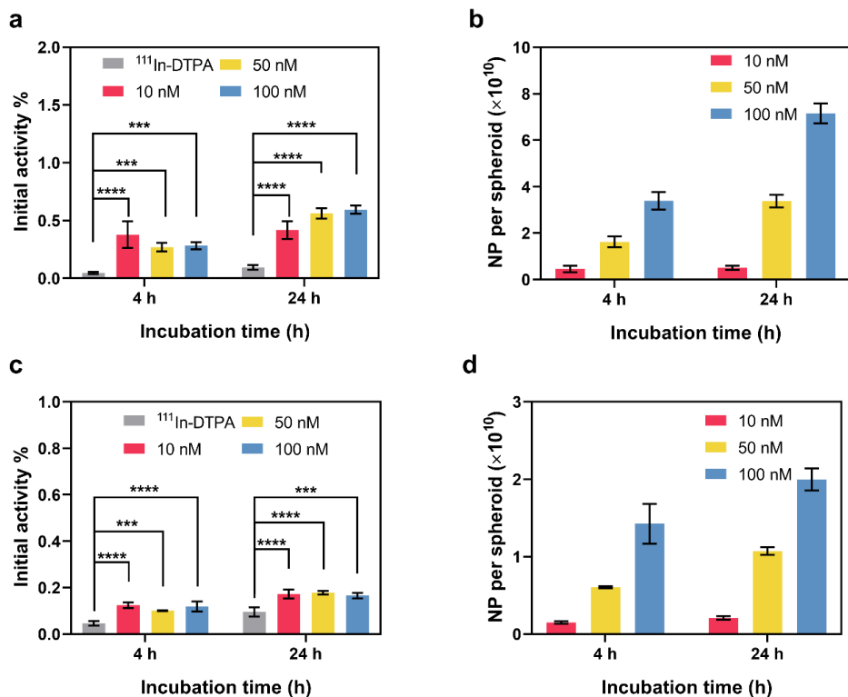
Figure 4.7. In vitro uptake of ^{111}\text{In-DTPA-AuNPs} (a-b) and ^{111}\text{In-DTPA-Ag}_2\text{TeNPs} (c-d) in 3D U87 spheroids for various nanoparticle concentrations and at incubation time of 4 or 24 h. The results are presented as percentage of the initially added activity (a and c) as well as nanoparticles per spheroid (b and d), n=4 .
