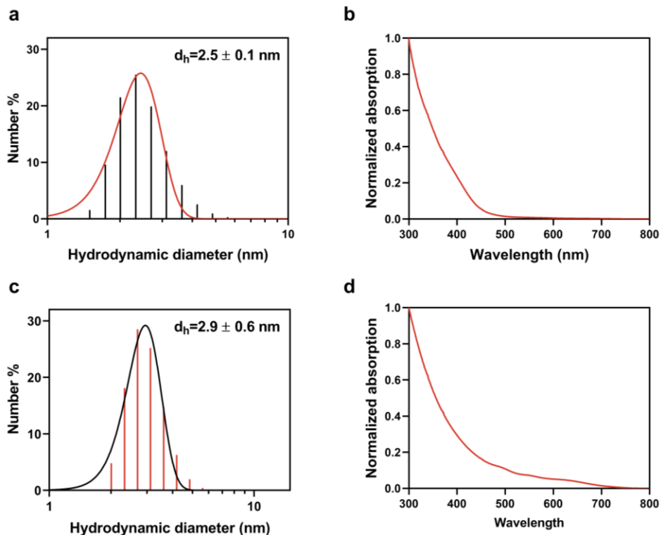
Figure S4.3. Number based hydrodynamic diameter of a) DTPA-AuNPs and c) DTPA- \text{Ag}_2\text{Te} NPs. Normalized UV-vis spectrum of b) DTPA-AuNPs and d) DTPA- \text{Ag}_2\text{Te} NPs. The nanoparticles were dispersed in PBS for the DLS and UV-vis measurements.
