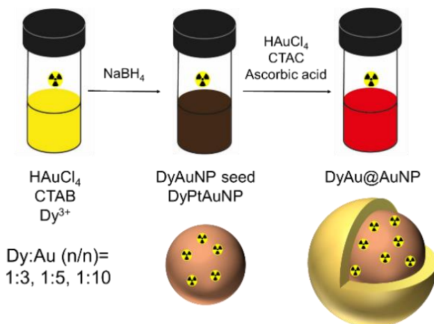
Figure 2.2. Schematic illustration of the synthesis of ^{166}\text{DyAu@AuNP} and ^{166}\text{DyPtAuNP} .
