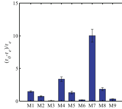
Fig. 5. Thixotropic index of AAS concretes.
