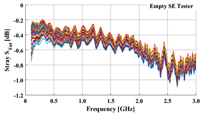
FIGURE 7. Total stray shielding measured fifty times after each unmounting and mounting of the empty SE Tester.
