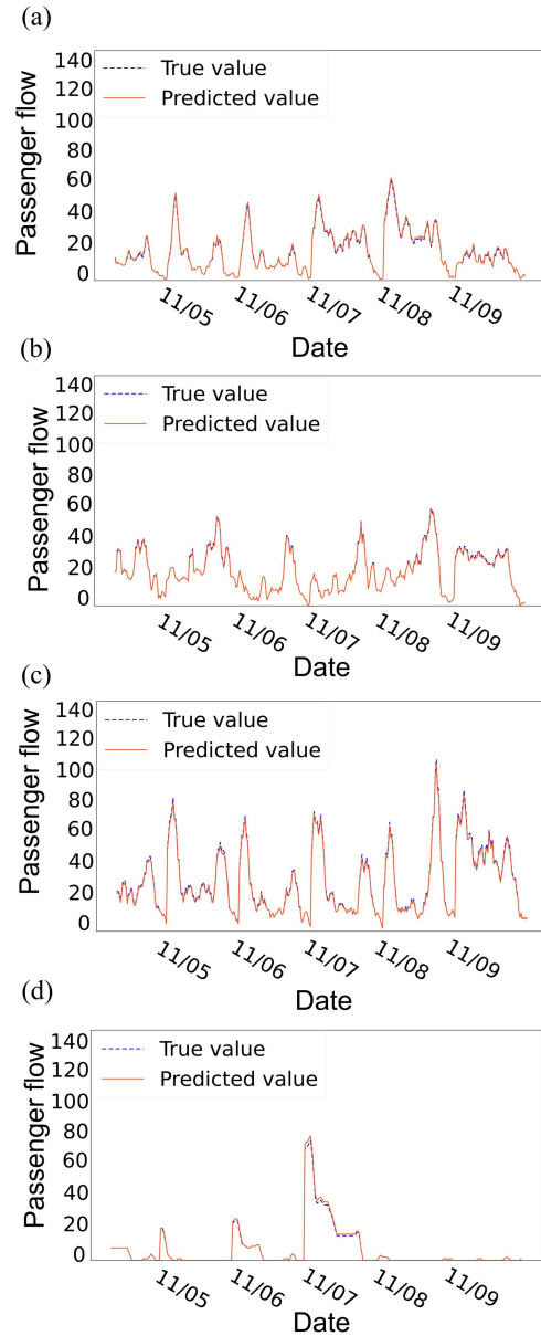
Fig. 15. The predicted results for four randomly chosen non-busy stations at one predicted step. (a) Predicted outflow v.s. the true value of Lianhua station at the first forecasting step. (b) Predicted outflow v.s. the true value of Liuxiandong station at the second forecasting step. (c) Predicted inflow v.s. the true value of Shenzhen Northern Railway station at the third forecasting step. (d). Predicted inflow v.s. the true value of Liyumen station at the fourth forecasting step.
