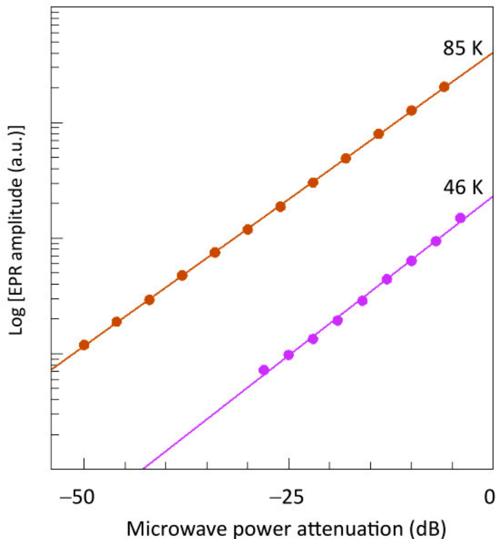
Figure 8. Power plots of the Y_2X_2 feature. The logarithm of the amplitude of the Y_2X_x feature at 85 K (brown) and 46 K (violet) is plotted versus the microwave power in dB attenuation from 200 mW. Linearity of the data shows that the signal does not saturate up to full power at the two temperatures.
