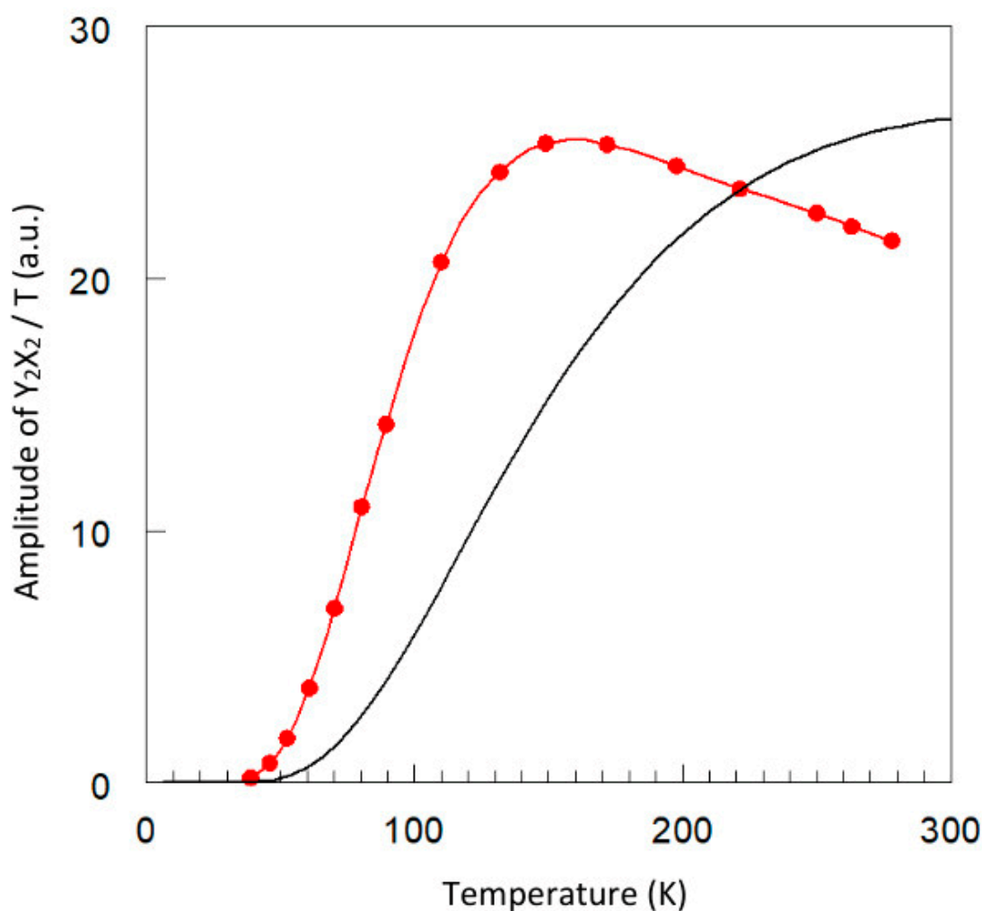
Figure 6. Comparison of triplet population level and normalized EPR intensity. The black line is the triplet population calculated with Equation (3). The red dots are real amplitudes of the spectra in Figure 5 divided by the absolute temperature. The red curve is a spline fit to the data. Its maximum is adjusted to that of the population curve. The shapes of the two curves differ because the red one is the result of depopulation combined with line sharpening with decreasing temperature. Its maximum, around 150 K, is taken as a compromise temperature for a broadband EPR study, because both signal-to-noise ratio and spectral resolution at this temperature are acceptable, and broadening of the Y_2 feature and the specific line shape of the X_2 feature at temperatures below 150 K are not understood (see also Figure 7).
