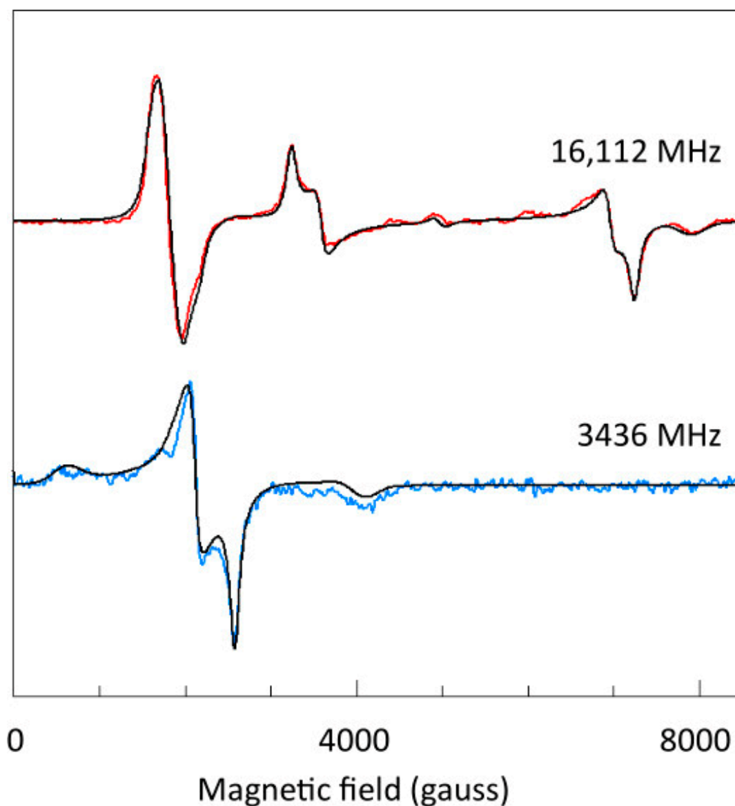
Figure 10. Simulation of triplet EPR spectra taken at two widely different frequencies. Simulation of the spectrum at 16,122 MHz with the program BB-TRIPLET was optimized by visual inspection, affording the parameters given in Table 1. Those parameters were then used without further optimization to generate a simulation of the spectrum at 3436 MHz. The fit indicates that the linewidths in x-, y-, and z-directions are fully independent of the microwave frequency. Experimental spectra were taken from Figure 9.
