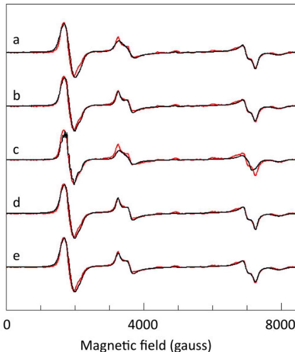
Figure 11. Exploration of contributions from different broadening mechanisms to the 150 K spectrum at 16.11 GHz. The simulations are as in Figure 10, top trace (where W_{zyx} = 85, 85, 70 gauss) plus additional broadening, and with the Lorentzian linewidth from spin-lattice relaxation concomitantly reduced. In trace (a), D strain, or a Gaussian distribution in D values, is introduced with a standard deviation \Delta D = 0.004 \text{ cm}^{-1} around the average value of D = 0.335 \text{ cm}^{-1} ( \Delta D \approx 1\% ), and W_{zyx} = 65, 65, 50 gauss.
