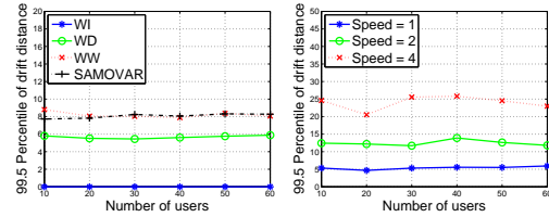
Fig. 11. Drift distance of AoS with: (left) different workloads and (right) WD workload and different movement speeds.
