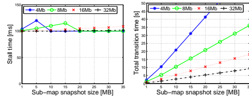
Fig. 15. UA to SA transitions with different sub-map sizes: (left) stall time and (right) total transition time.
