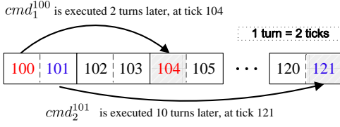
Fig. 19. Dynamic delay-execution.
