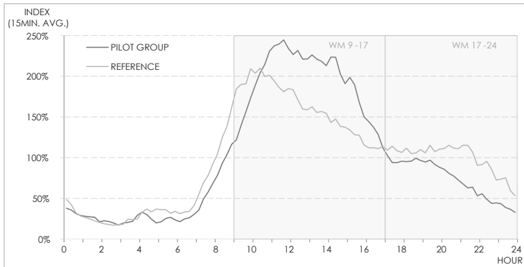
FIG. 6.5 AVERAGE LOAD PROFILES OF THE WASHING MACHINE FOR THE PILOT GROUP VS. THE REFERENCE GROUP
