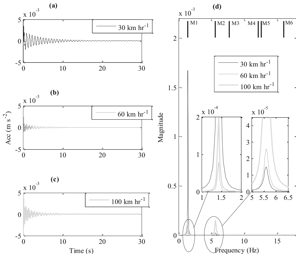
Fig. 11 Free vibration only— sensor S2. a Free vibration measured after vehicle traversed at 30 km h -1 ; b free vibration measured after vehicle traversed at 60 km h -1 ; c free vibration measured after vehicle traversed at 100 km h -1 ; d frequency content of signals in (a–c)
