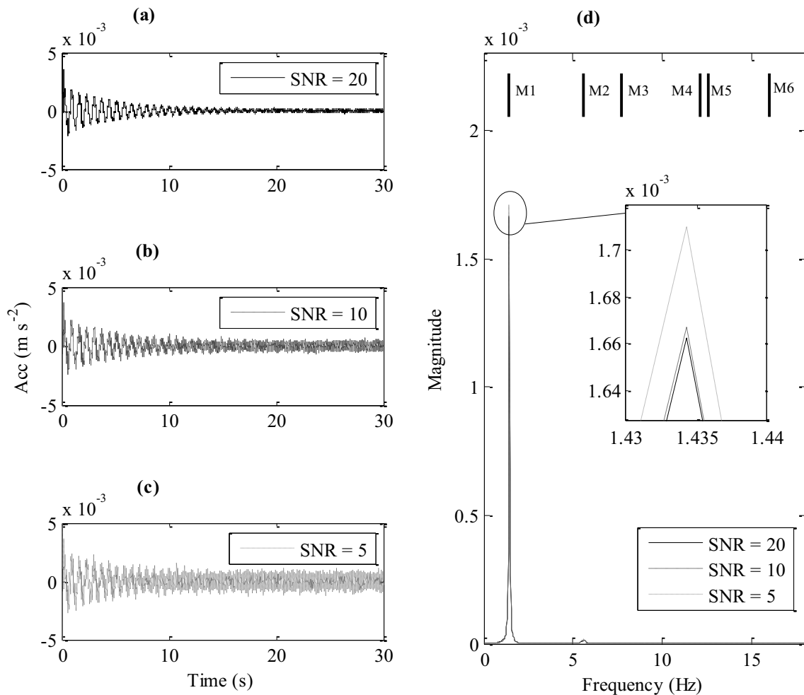
Fig. 14 Effect of added noise on frequency clarity—free vibration at sensor S2 after vehicle traverses at 30 km h -1 , a SNR = 20, b SNR = 10, c SNR = 5, d frequency of signals in (a) to (c) ( inset ) zoomed in at peak of frequency
