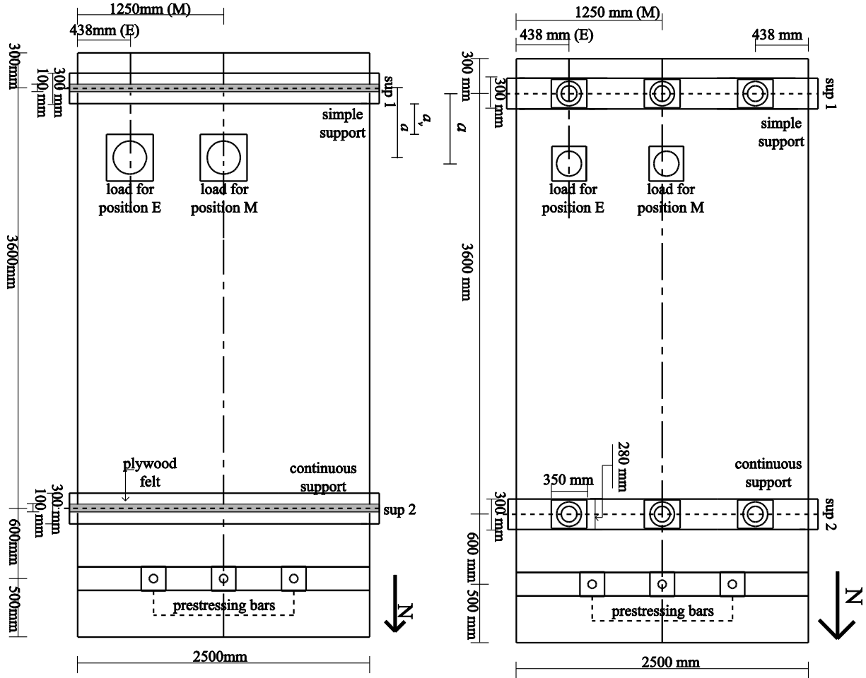
10 Figure 2 – Test setup for slab shear experiments: (a) with line supports; (b) supported by elastomeric 11 bearings. Units: mm; 1 mm = 0.04 in.
