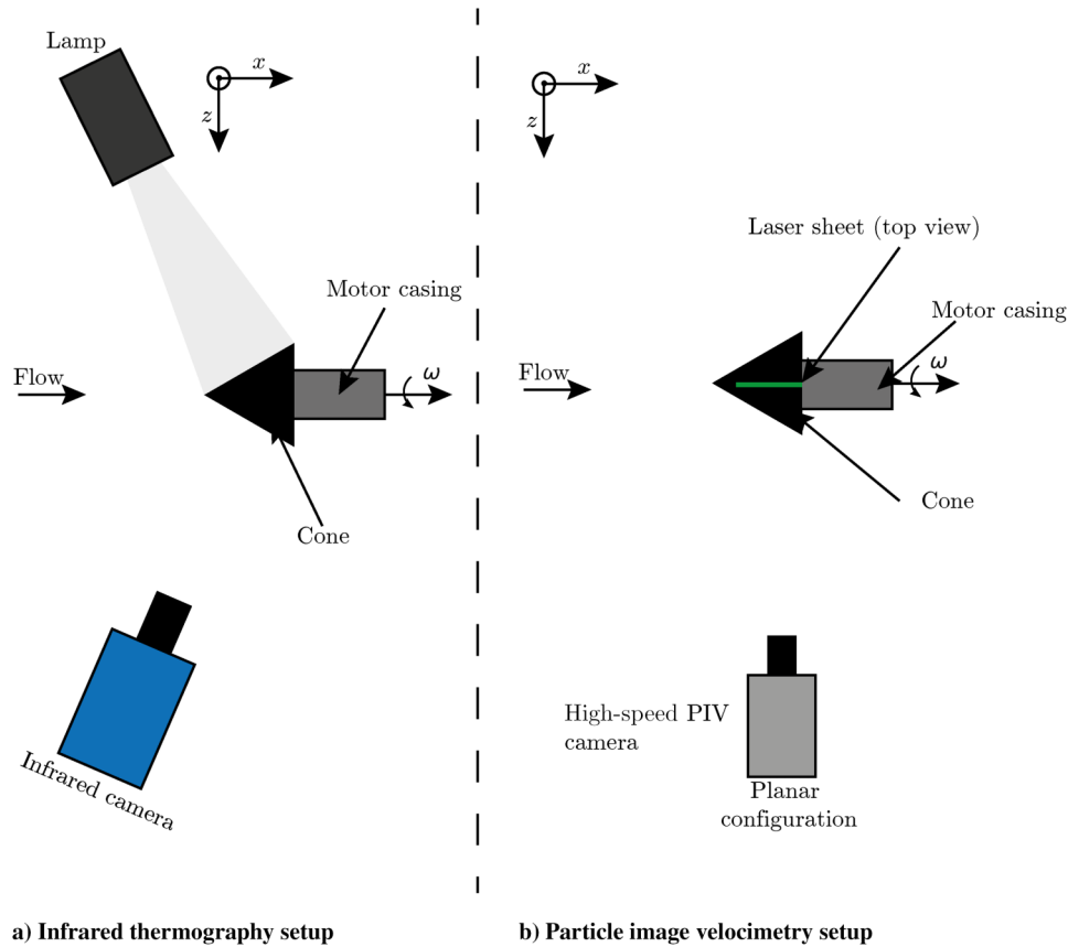
Fig. 2 Schematic of the experimental arrangements: a) infrared thermography and b) particle image velocimetry.
