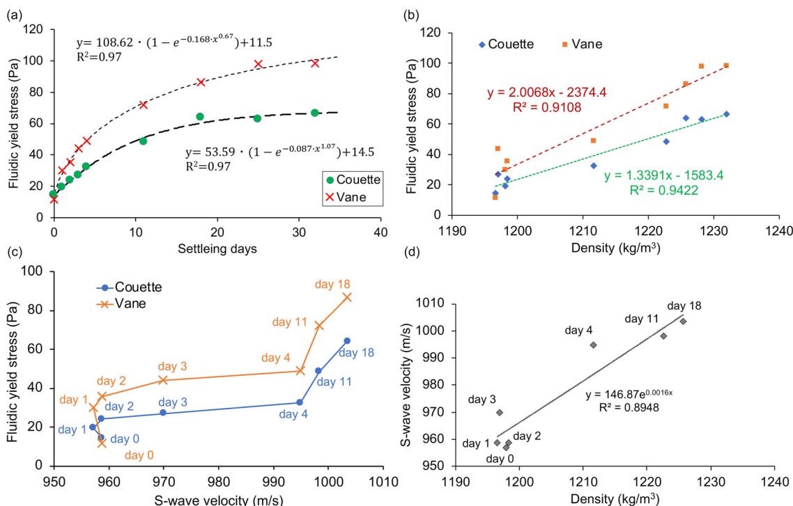
FIG. 9. (Color online) (a) The temporal change of the fluidic yield stress using measurements with the Couette [Fig. 8(a)] and vane geometries [Fig. 8(b)]. The point measurements are fitted using regression analysis. (b) The fluidic yield stress versus density using measurements of the Couette and vane geometries. (c) The fluidic yield stress versus S-wave velocity using measurements the Couette and vane geometries. (d) The S-wave velocity versus density.
