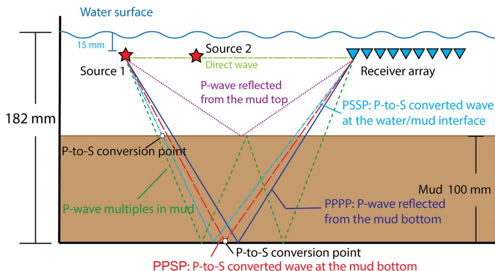
FIG. 1. (Color online) Sketch of the reflection-measurement geometry and travelpaths of the different expected wave-type arrivals. The travelpaths are only illustrative and do not represent the actual propagation travelpaths.
