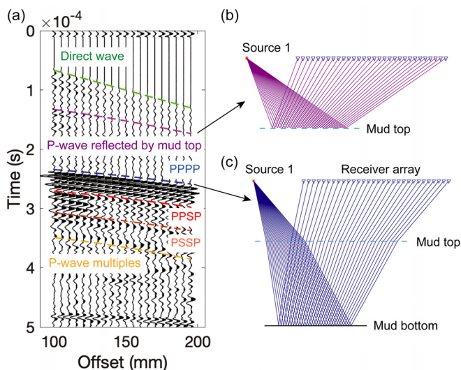
FIG. 3. (Color online) (a) The recorded common-source gather due to source 1. The different interpreted arrivals are the direct wave (green); P-wave reflected from the mud top (magenta); P-wave reflected from the mud bottom, labeled PPPP (blue); its first-order internal multiple (yellow); P-to-S conversion at the mud bottom, labeled PPSP (red); and P-to-S conversion at the water/mud interface, labeled PSSP (orange). (b) The Common-source gather recording illustrating pseudo-travelpaths reflected by the mud top. (c) As in (b) but reflected by the mud bottom.
