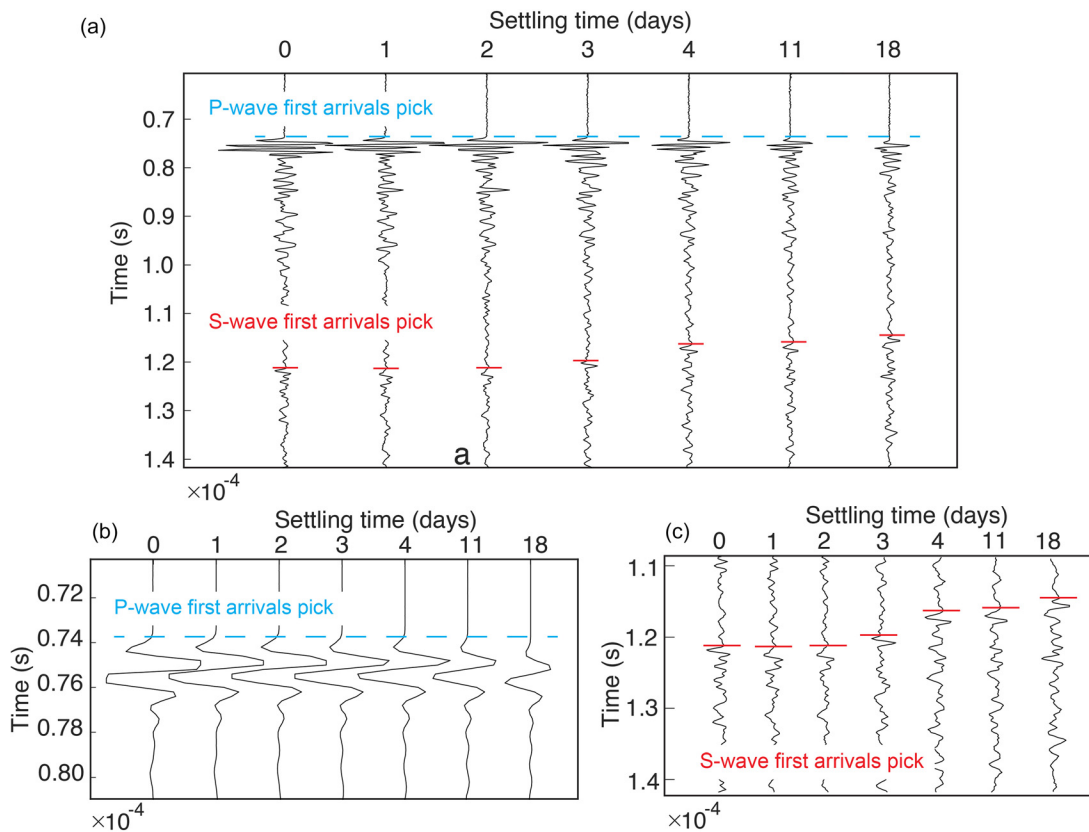
FIG. 6. (Color online) (a) The arrival time of the direct P- and S-waves using seismic transmission measurements during the settling process. Zoomed in sections of the recordings in (a) around the first arrivals of (b) the P-wave and (c) the S-wave.
