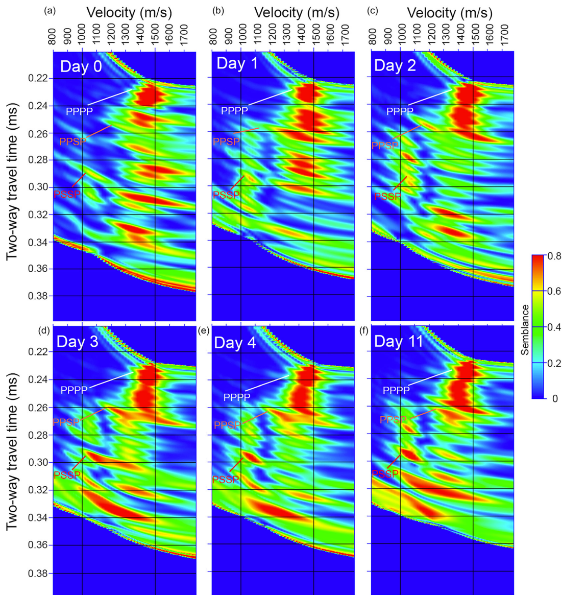
FIG. 10. (Color online) The temporal changes of the seismic reflections PPPP, PPSP, and PSSP from the fluid mud and water layer obtained from the semblance analysis of the common-source reflection gathers measured at (a) day 0, (b) day 1, (c) day 2, (d) day 3, (e) day 4, and (f) day 11.
