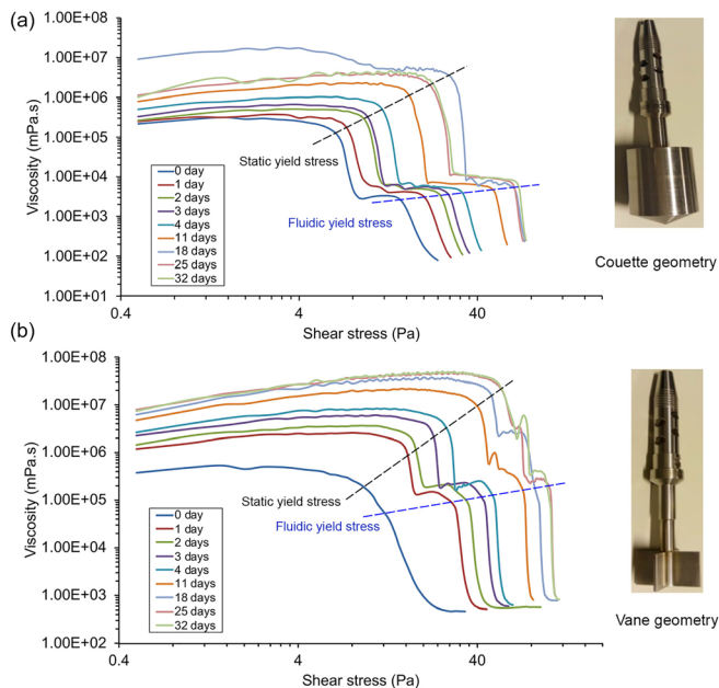
FIG. 8. (Color online) (a) The apparent viscosity versus stress obtained using measurements with the Couette geometry. (b) As in (a) but with vane geometry.
