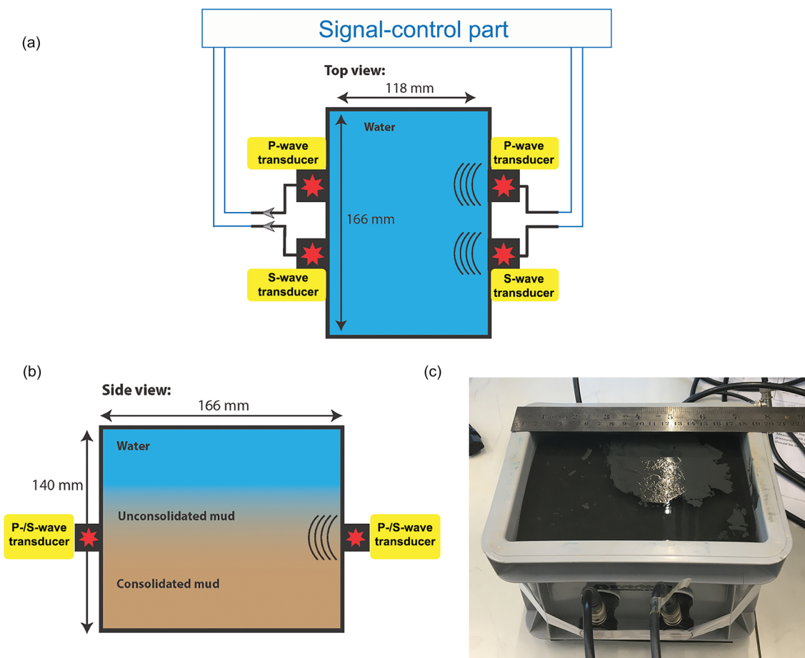
FIG. 5. (Color online) (a) Sketch of the seismic-transmission measurement system showing the top view of a box containing water and fluid mud, to which are attached ultrasonic transducers. (b) Sketch of the side view of the box with the ultrasonic transducers. (c) The photo of the actual box and transducers installed on it.
