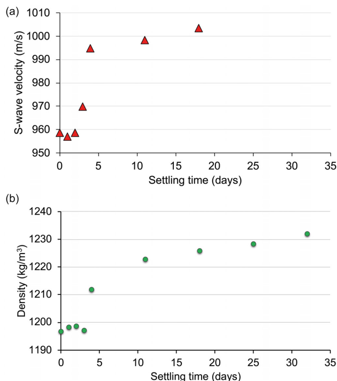
FIG. 7. (Color online) (a) The time-lapse evolution of the S-wave velocity with the settling time estimated using the seismic transmission measurements. (b) The temporal change of the density of the fluid mud with the settling time.
