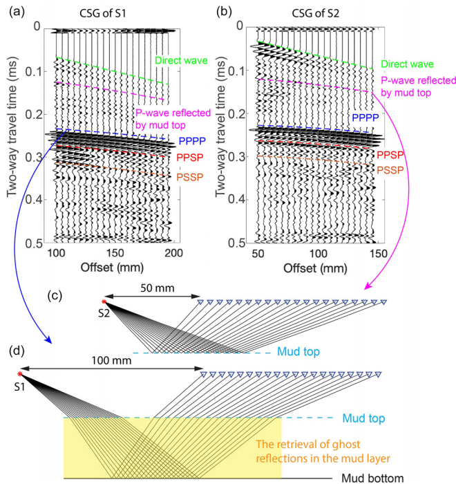
FIG. 11. (Color online) The reflection common-source gathers (CSGs) from (a) source 1 and (b) source 2 used for retrieval of a ghost reflection inside the mud layer. Sketch of (c) the travelpaths of the P-waves reflected by the mud top in CSG from S2 and (d) the travelpaths of PPPP in CSG from S1. The highlighted part in (d) shows the parts of the wavefield contributing to the retrieval of the ghost reflection. The PPSP and PSSP arrival waves have similar structures to those of PPPP and, thus, the retrieval process is essentially the same.
