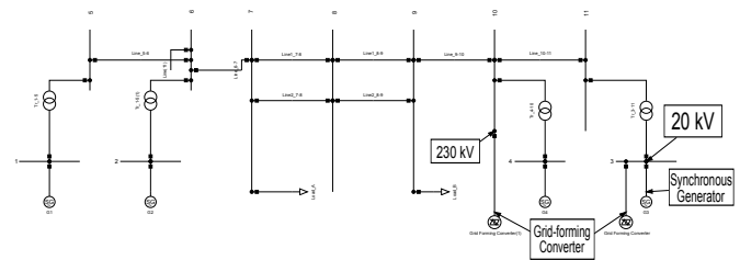
Fig. 1. System schematic in Powerfactory
