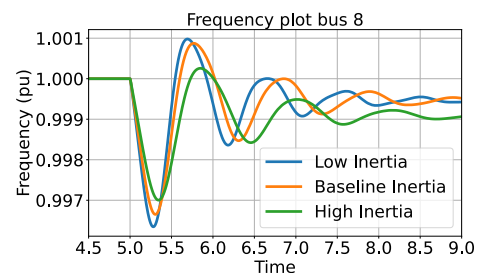
Fig. 7. Frequency plot representing increased and reduced level of inertia during perturbation
