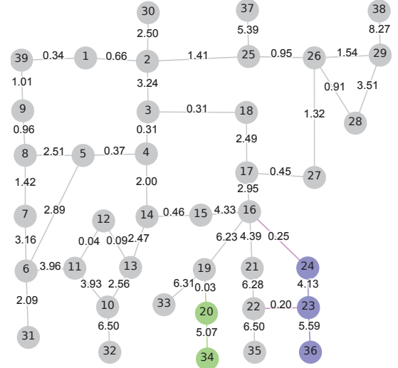
Figure 1: Active power flow graph of the IEEE 39 bus test system obtained by perturbing the loads around the nominal value. The edge weights represent the active power flows in p.u. on the 100 MVA base.
