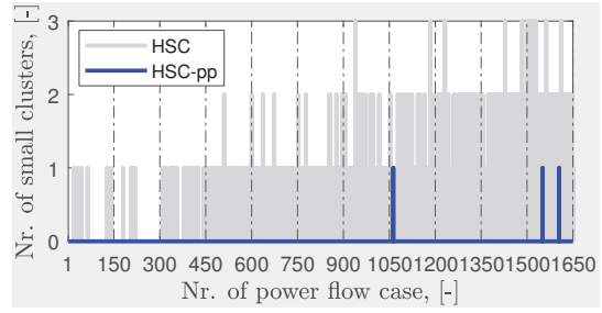
(b) case1354pegase test network
