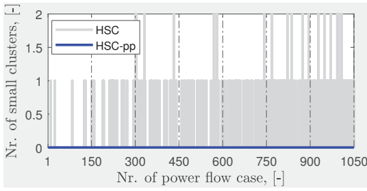
(a) case300 test network
