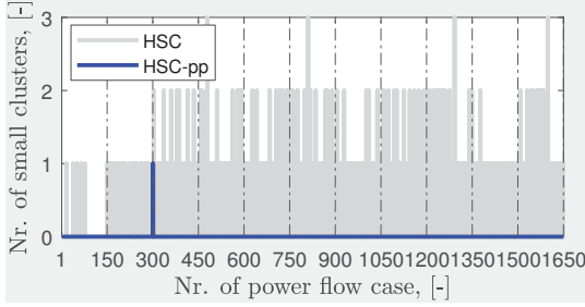
(c) case2383wp test network
