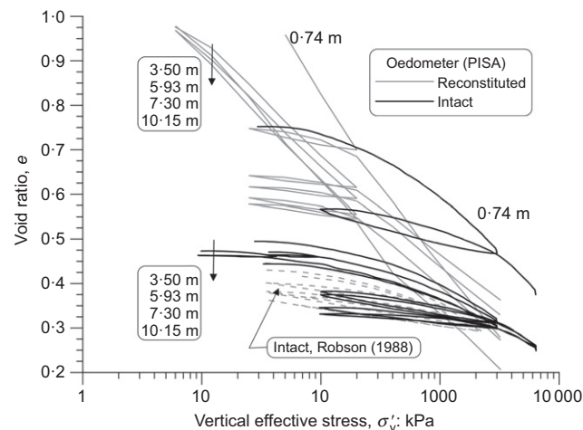
Fig. 6. One-dimensional compression of Cowden till samples
