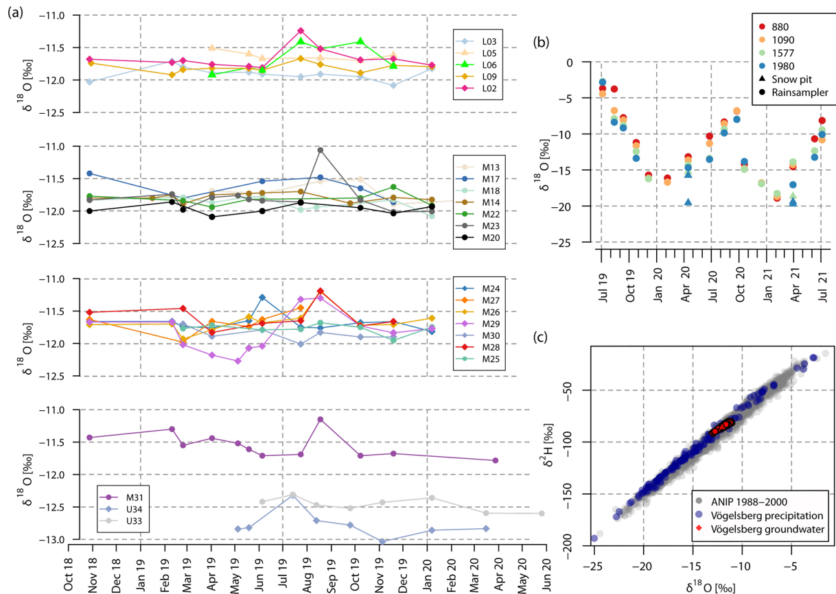
Figure 7. Time series of \delta^{18}\text{O} of selected springs (a), time series of \delta^{18}\text{O} in precipitation (b), and \delta^{18}\text{O} vs. \delta^{2}\text{H} in precipitation (ANIP and Vögelsberg) and groundwater (Vögelsberg) (c).
