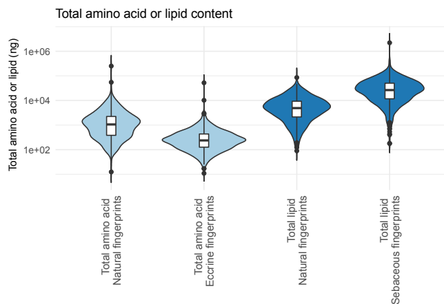
Fig. 1. The distribution of total amino acid and lipid content (ng) in the natural, eccrine and the sebaceous fingerprints, calculated as sum of all quantified amino acids (LC-MS) or lipid compounds (GC-MS).
