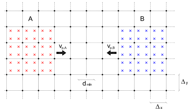
Fig. 4. Collision benchmark.
