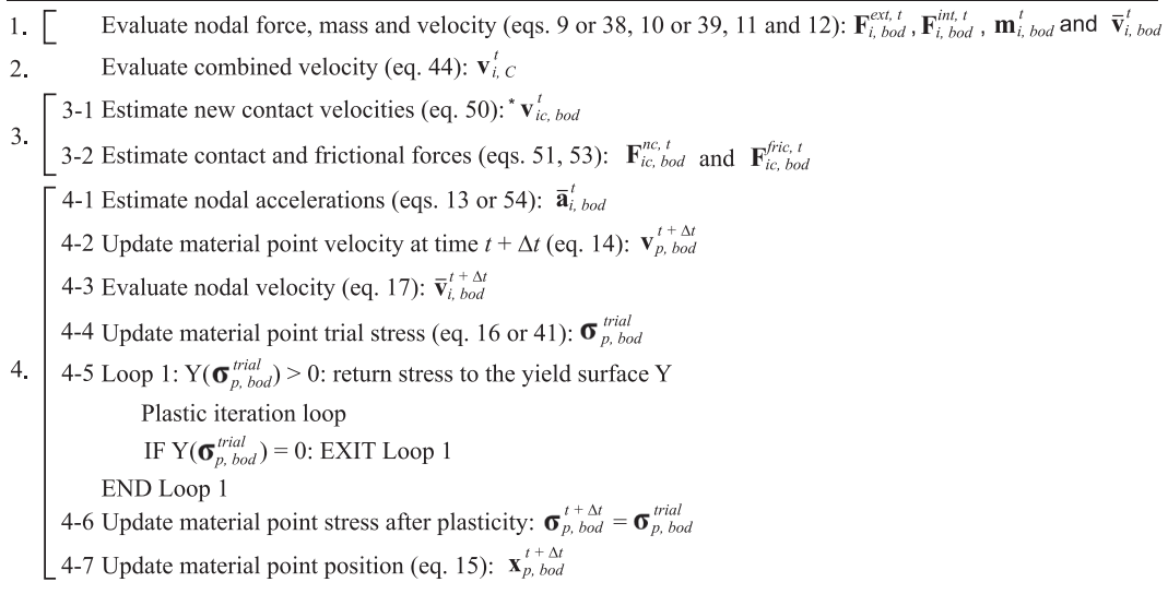
Fig. 2. Steps followed in the explicit solution scheme, in which the square brackets indicate a loop over the bodies.
