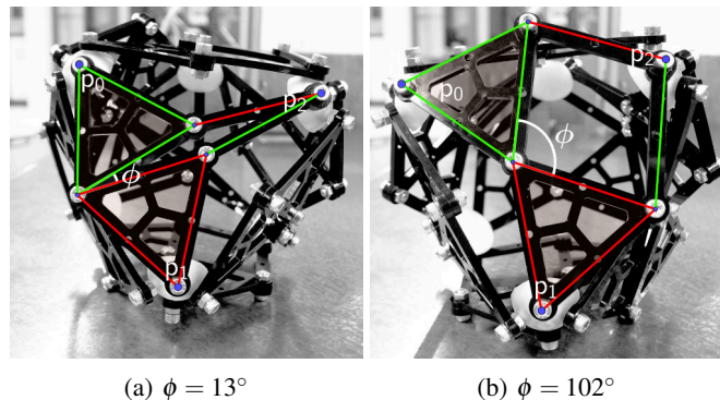
Fig. 9: Two faces of the octahedron in the compacted state. The lines drawn on top were used to estimate the angle \phi in this configuration, the labels p_0, p_1, p_2 refer to the points drawn in fig. 2
