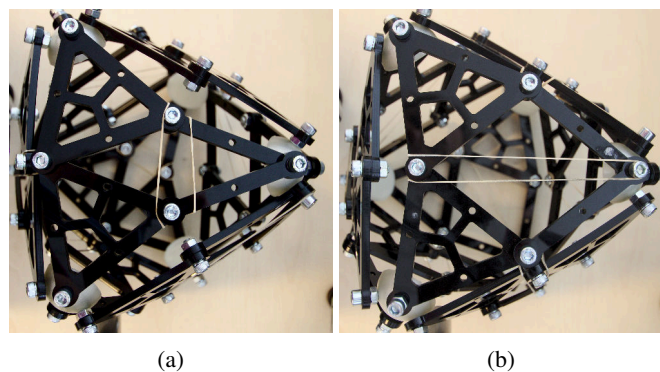
Fig. 10: Two faces of the octahedron with rubber bands applied to change the lowest-energy configuration to a non-singular one.
