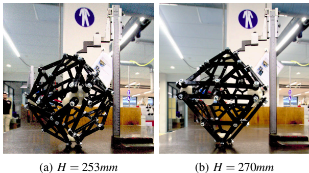
Fig. 8: Measurements of the distance between two opposing vertices of the octahedral structure. The measured heights are given in the subcaptions.
