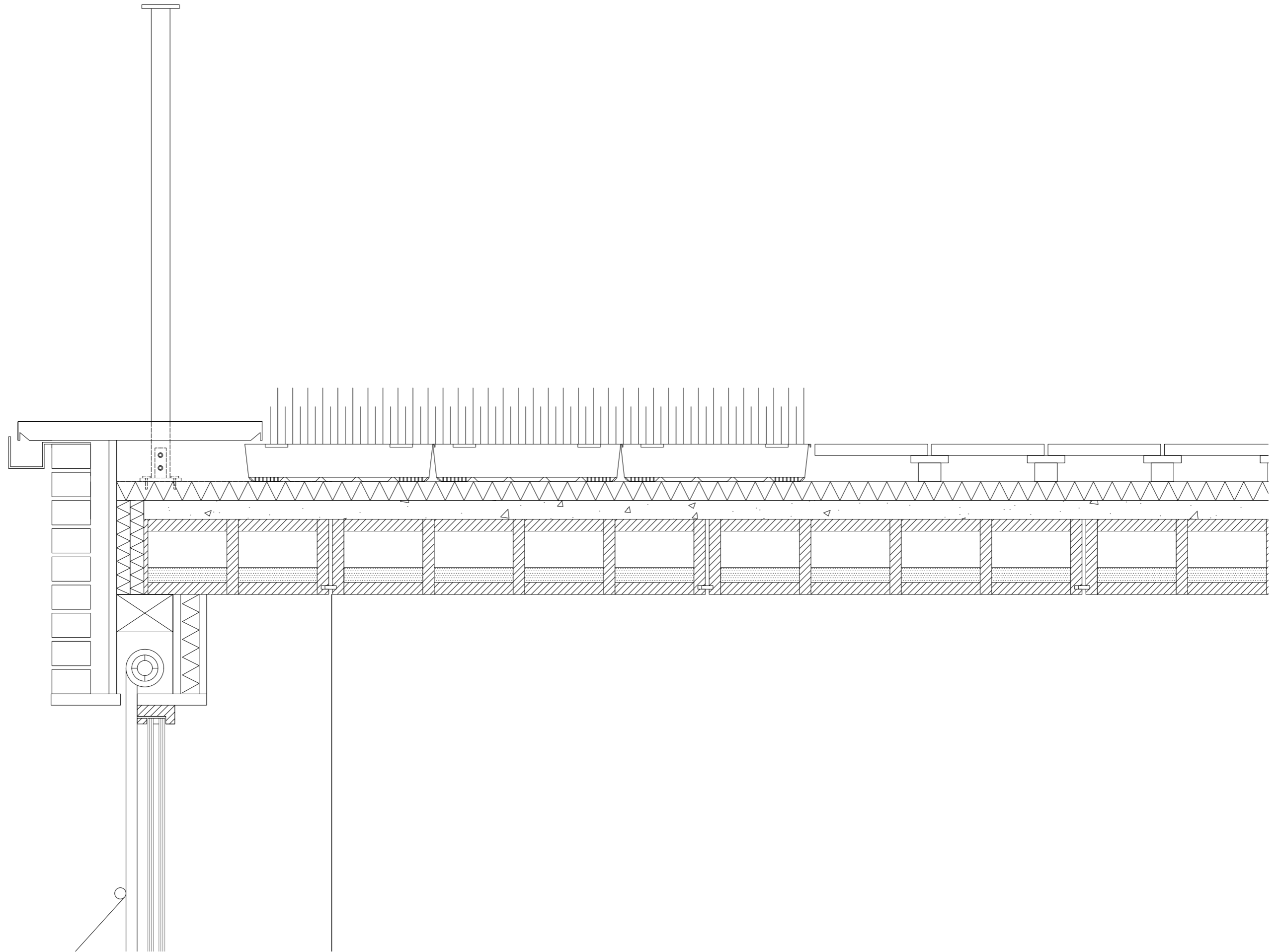
Wall to roof connection 1/10
