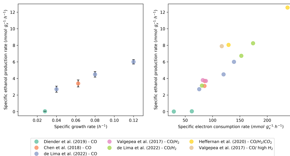
Figure 2.2: Dependency of the biomass-specific ethanol production rate ( q_{EtOH} ) on specific growth- and electron uptake rate of C. autoethanogenum . Panel A: q_{EtOH} data was obtained from three independent studies [32–34] and plotted as a function of the reported \mu . All studies were performed in gas-liquid mass transfer-limited continuous cultures fed with CO as only carbon- and electron source, either in chemostat or in a bubble column. One study [34] was executed at higher pH than the other two studies (6.2 vs 5). Low pH is known to trigger solventogenesis [20], which may explain the slight diversion of q_{EtOH} in this study as compared to the trend through the other datasets. Panel B: chemostat studies fed with mixtures of CO, H 2 and CO 2 were compiled by plotting the electron uptake rate ( \sum(q_{CO} + q_{H_2}) \cdot 2 ) versus the observed ethanol production rate. Seven different datasets of continuous cultures with C. autoethanogenum were included in this analysis [4, 31–35].
