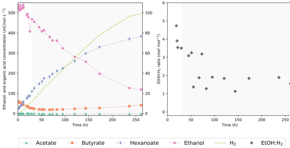
Figure 5.4: Biochemical conversion profiles (A) and \text{EtOH:H}_2 ratios (B) during ethanol chain elongation in presence of butyrate. 100 mL of an active chain-elongating community was incubated in a batch bioreactor with 300 mM ethanol and 15 mM butyrate. Different phases in the experiment are distinguished with different shades of background color. \text{EtOH:H}_2 ratios were calculated using the point-wise difference between consumed ethanol and produced hydrogen. Due to fluctuating ethanol measurements in the first 21 hours, the \text{EtOH:H}_2 ratio in this phase was calculated from t=0 to t=19 and from t=0 to t=20.5 with the initial concentration of ethanol as reference. Solid lines are linear interpolations between the data points.
