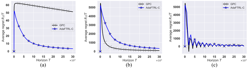
Figure 1: Average regret when (a): \boldsymbol{\theta}_t = (1, 1), \mathbf{w}_t = -(0.1, 0.1) \forall t ; (b): \boldsymbol{\theta}_t = (10, 10), \mathbf{w}_t = -(1, 1) \forall t ; (c): \boldsymbol{\theta}_t = (10, 10) or -(10, 10) (Alternating every 1000 steps), \mathbf{w}_t = -(1, 1) \forall t .
