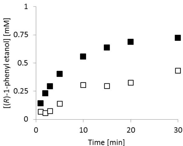
Figure 13. rAaeUPO catalyzed hydroxylation of ethyl benzene to phenyl ethanol upon addition of 1 mM of \text{H}_2\text{O}_2 , with the enzyme either in a dialysis bag (white) or free in solution (black). The reaction mixtures were equally divided inside as outside the bag. Conditions for the physically separated reaction: Inside the bag: [ethyl benzene] = 50 mM, [ rAaeUPO ] = 100 nM, KPi buffer pH 7.0 (100 mM). Outside the bag: [ \text{H}_2\text{O}_2 ] = 2 mM, [ethyl benzene] = 50 mM, KPi buffer pH 7.0 (100 mM). Conditions for the free enzyme reaction: [ethyl benzene] = 50 mM, [ \text{H}_2\text{O}_2 ] = 1 mM, [ rAaeUPO ] = 50 nM, KPi buffer pH 7.0 (100 mM). The single reactions were performed at room temperature while magnetically stirring at 600 rpm.
