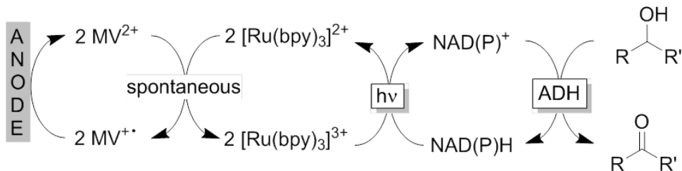
Scheme 11. The photoelectrochemical NAD(P) + regeneration system proposed by Steckhan and coworkers to promote ADH-catalysed oxidation reactions.
