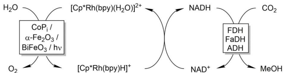
Scheme 5. Coupling photochemical water oxidation to enzymatic CO 2 reduction. The photocatalytic cascade comprises BiFeO 3 as photoactive catalyst transferring electrons to [\text{Cp}^*\text{Rh}(\text{bpy})(\text{H}_2\text{O})]^{2+} . The electrons are obtained from water by co-catalysis of cobalt phosphate (CoPi) and \alpha\text{-Fe}_2\text{O}_3 . The reduced Rh-complex specifically transfers NAD + into NADH, which drives the reduction of CO 2 to MeOH through a cascade of formate dehydrogenase (FDH), formaldehyde dehydrogenase (FaDH) and alcohol dehydrogenase (ADH).
