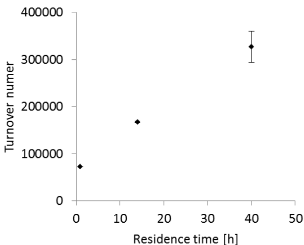
Figure 4: Increasing the PeAAOx turnover numbers (TN) in flow by increasing the residence time. Conditions: 6 ml flow reactor, [trans\text{-}2\text{-hexenol}]_0 = 40 mM, [PeAAOx] = 0.02 \mu M, [catalase] = 600 U ml^{-1} in a 50 mM KPi buffer (pH 7.0) at 30 °C. The TN value was calculated based on the GC yield of every run. The TN was obtained by dividing the product concentration (as determined chromatographically) by the biocatalyst concentration.
