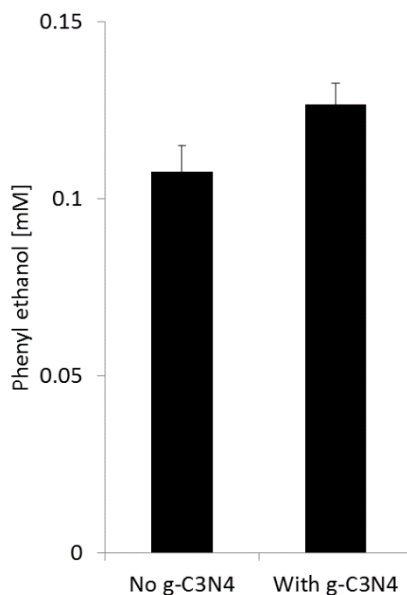
Figure 11. The effect of g\text{-C}_3\text{N}_4 on rAaeUPO in absence of the light source. 10 nM rAaeUPO in KPi buffer (100 mM, pH 7.0) was incubated in presence or absence of 5\text{ mg ml}^{-1} of g\text{-C}_3\text{N}_4 for 13 hours at 30\text{ }^\circ\text{C} . Thereafter, 50 mM ethyl benzene and 1 mM were added to all samples and the reaction was run of 30 minutes. Reaction solutions were extracted with ethylacetate and subsequently analysed on GC. Experiments were performed in triplicates.
