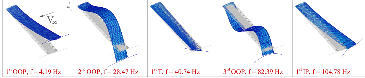
Fig. 4 Lowest five natural mode shapes as computed by MSC Nastran of the undeformed Pazy Wing full FEM with skin (OOP = Out-of-Plane bending, T = Torsion, IP = In-Plane bending).
