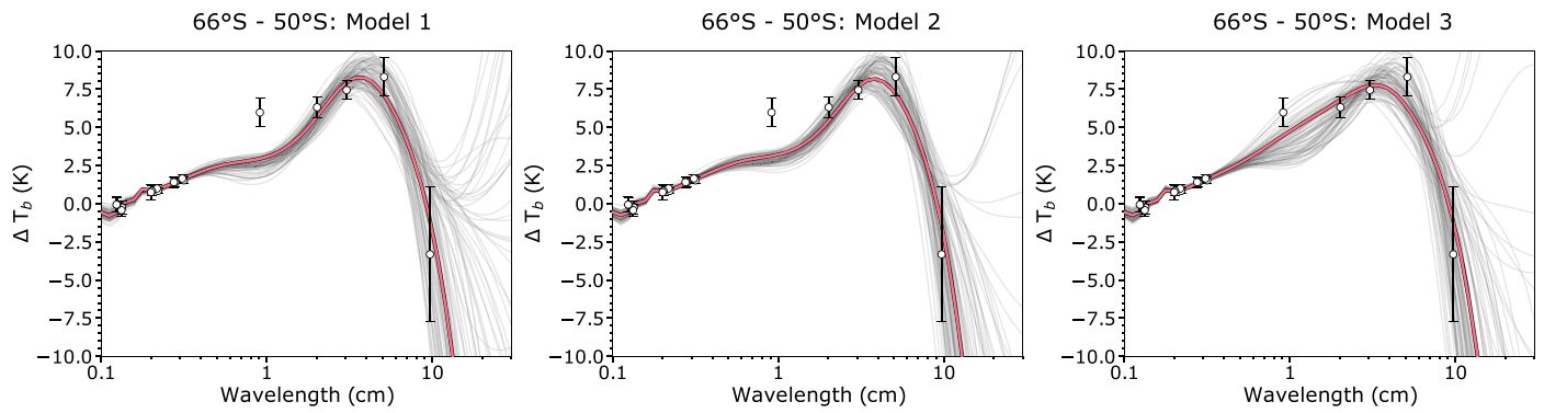
Figure A4. Random retrieved model spectra fitting the observed \Delta T_b between 66^\circ\text{S} – 50^\circ\text{S} and 36^\circ\text{S} – 12^\circ\text{S} for the three types of models considered in this section. Only model 3, which allows \text{H}_2\text{S} supersaturation at its ice cloud, provides a good fit to the data at 0.9 cm.
