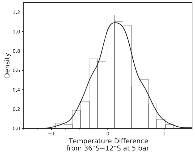
Figure A6. Distribution of retrieved kinetic temperature differences between 66^\circ\text{S} – 50^\circ\text{S} and 36^\circ\text{S} – 12^\circ\text{S} at 5 bar for model 3. Differences are consistent with zero and are no larger than 1 K.
