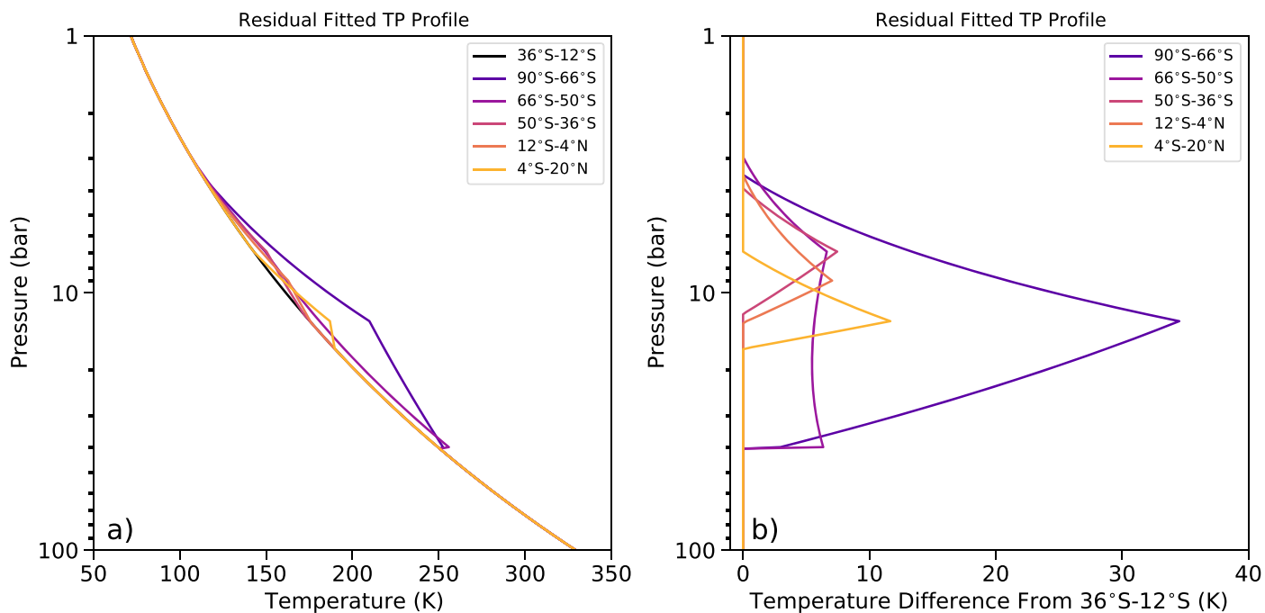
Figure A2. (a) Temperature profiles as a function of latitude (colored lines) producing the residual spectra fits plotted in Figure A1. (b) Residual temperature profile as a function of latitude (colored lines), where the 36°S–12°S dry adiabat profile is subtracted from the temperature at the given latitude band.
