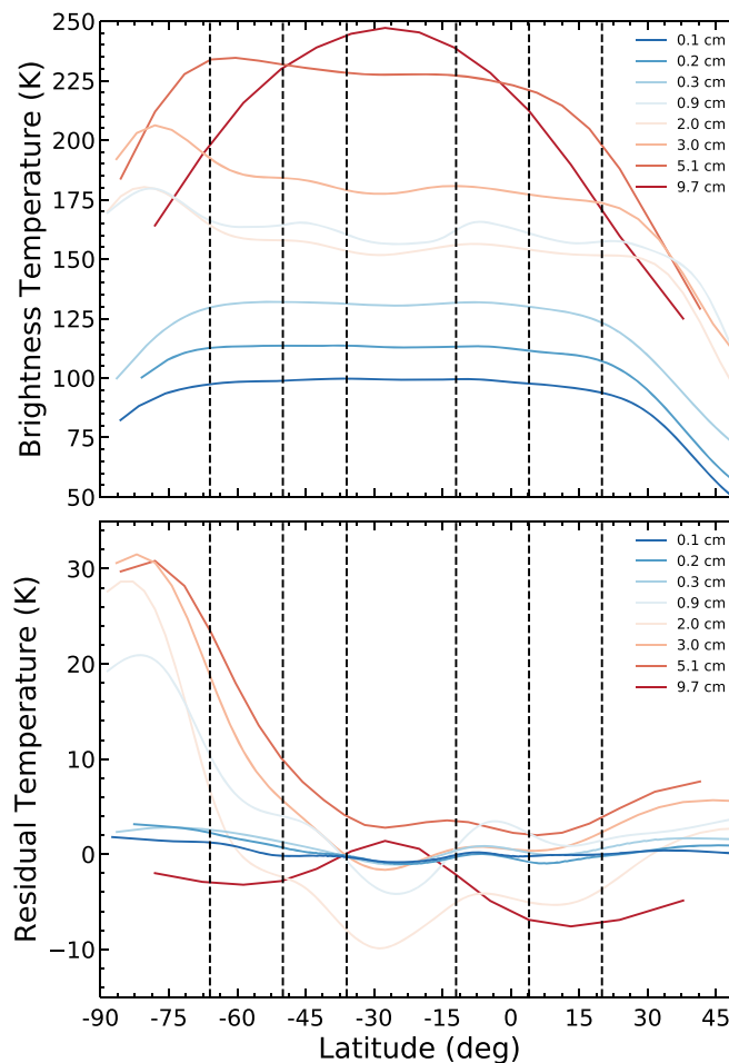
Figure 2. Neptune’s observed brightness temperature (top panel) and residual temperature (bottom panel) vs. latitude along the sub-observer longitude for each wavelength band (colored lines). The residual temperatures are taken from the residual maps shown in Figure 1 and are obtained by subtracting the observed brightness temperatures from best-fitting uniform limb-darkened disks, as described in Section 2.2 Dashed black lines delineate regions where brightness temperature variations are evident and define the latitude bins used in our modeling. Lines may not extend to 90°S due to limits in the resolution of the observation. The bump in the residual temperature at 9.7 cm is due to the poor resolution, as the large beam size impacts the limb-darkened fit.
