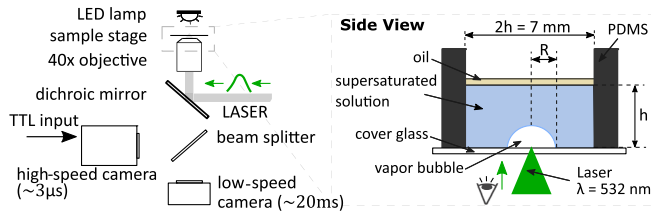
FIG. 1. Sketch of the experimental setup to generate a microbubble. The setup construction is detailed in our previous work [55]. The green arrow indicates the direction of laser pulse. PDMS: polydimethylsiloxane. TTL: transistor-transistor logic signal.
