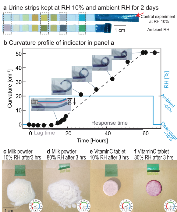
Figure 2. Demonstration on how the EHI (pointed out by red arrow) reports exposure to the elevated humidity by mechanical deformation. Panel (a) presents two EHI-attached urine strips stored under different humidity conditions after 2 days. After 2 days, the ability of the strips to fulfill their function is validated by identical artificial urine solutions. The strip at the top is the control sample stored at the recommended humidity level of 10% RH and gives the correct reading. However, the strip at the bottom, which is exposed to ambient conditions (fluctuating between 48% and 64% RH), gives a false reading evident from the color change distinct from the control (highlighted in gray). Panel (b) shows the curvature development of the EHI attached to the urine strip exposed to undesired ambient humidity conditions in panel (a) bottom. The dashed line is a guide for the eye. (c) Milk powder: 10% RH; 3 h in desiccator. (d) Milk powder: 80% RH; 3 h. (e) Vitamin C tablet: 10% RH; 3 h in desiccator. (f) Vitamin C tablet: 80% RH; 3 h. Moisture exposure diagnosed by a rolled EHI while there was no EHI bending in the control (desiccator-stored) experiments.
