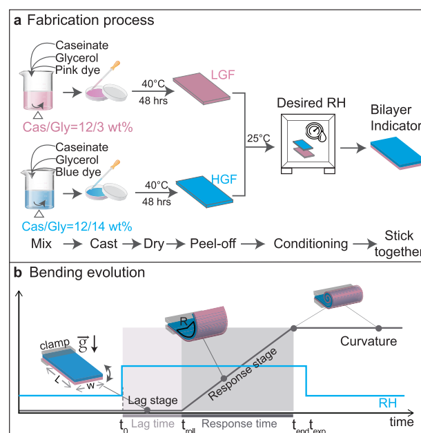
Figure 1. (a) Schematic representation of the fabrication process of the edible humidity indicator (EHI). (b) The flat EHI bends and rolls on itself to report humidity exposure. The bending evolution is irreversible and exhibits two stages including Lag stage and Response stage , which is schematically shown in the zoom plot (bottom). Figure not drawn to scale.
