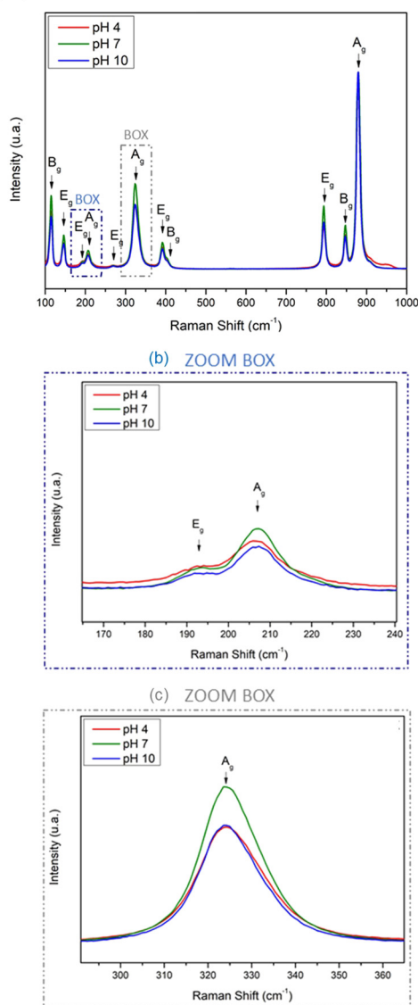
Fig. 5 Raman spectroscopy of samples synthesized at 100 °C, (a) samples with pH 4, 7 and 10, (b) zoomed-in box of modes E g and A g , and (c) zoomed-in box of mode A g .
