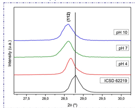
Fig. 4 XRD patterns of the sample synthesized at 140^\circ\text{C} . (a) Samples with pH 4, 7, and 10 and (b) zoomed plot of the range close to the (112) peak.
