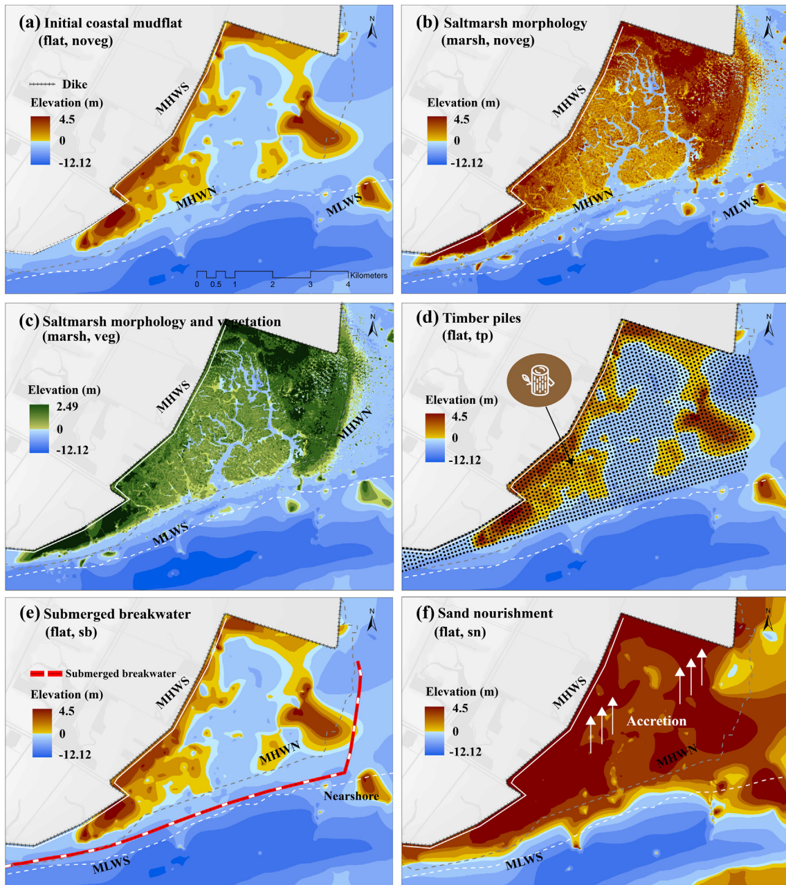
Fig. 4. Bathymetries and the scenario designs of the Nature-Based Flood Defense (Nbfd) measure. (a) The scenario of initial coastal mudflat (flat,novveg) , (b) The saltmarsh morphology (marsh,novveg) , (c) The scenario of saltmarsh morphology with attached vegetation (marsh,veg) , (d) The scenario of timber piles (flat,tp) , (e) The scenario of submerged breakwater (flat,sb) , (f) The scenario of sand nourishment (flat,sn) .
